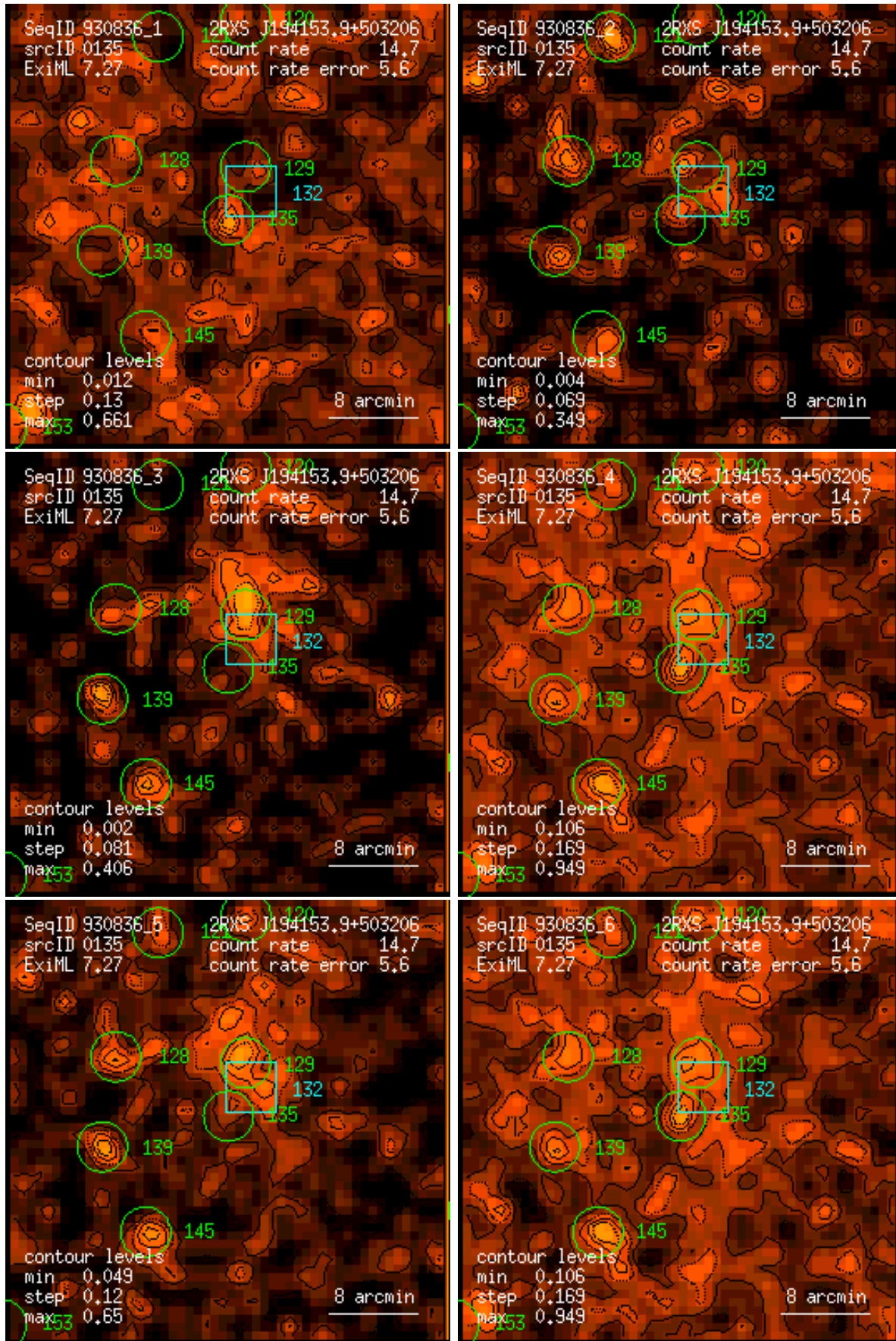
Figure 135: RASS 930836: detection 0135: band rate images, Gaussian filter: (1) PSPC channels 11 – 41, (2) 52 – 90, (3) 91 – 201, (4) 11 – 235, (5) 52 – 201, (6) 11 – 201. Broad band rates in counts/ks. Band rate contour levels in counts/ks/arcmin 2 .
