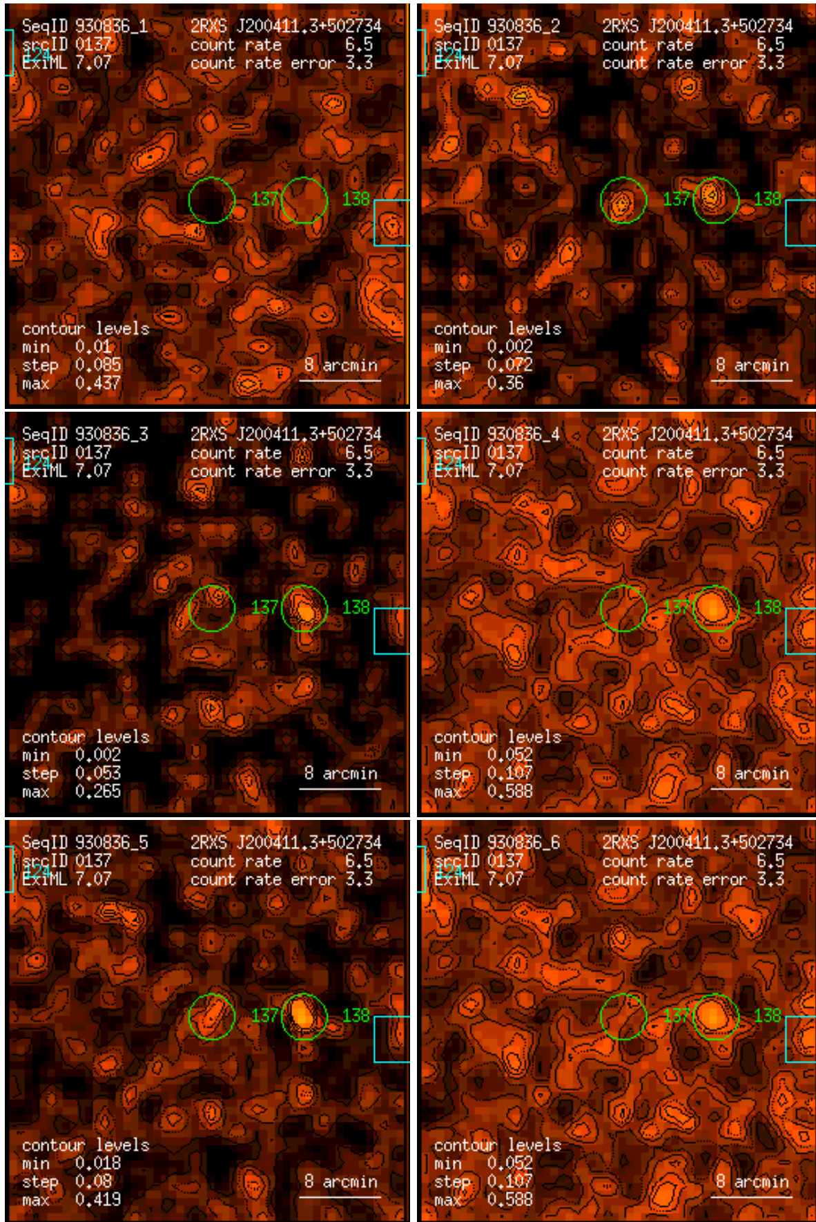
Figure 137: RASS 930836: detection 0137: band rate images, Gaussian filter: (1) PSPC channels 11 – 41, (2) 52 – 90, (3) 91 – 201, (4) 11 – 235, (5) 52 – 201, (6) 11 – 201. Broad band rates in counts/ks. Band rate contour levels in counts/ks/arcmin 2 .
