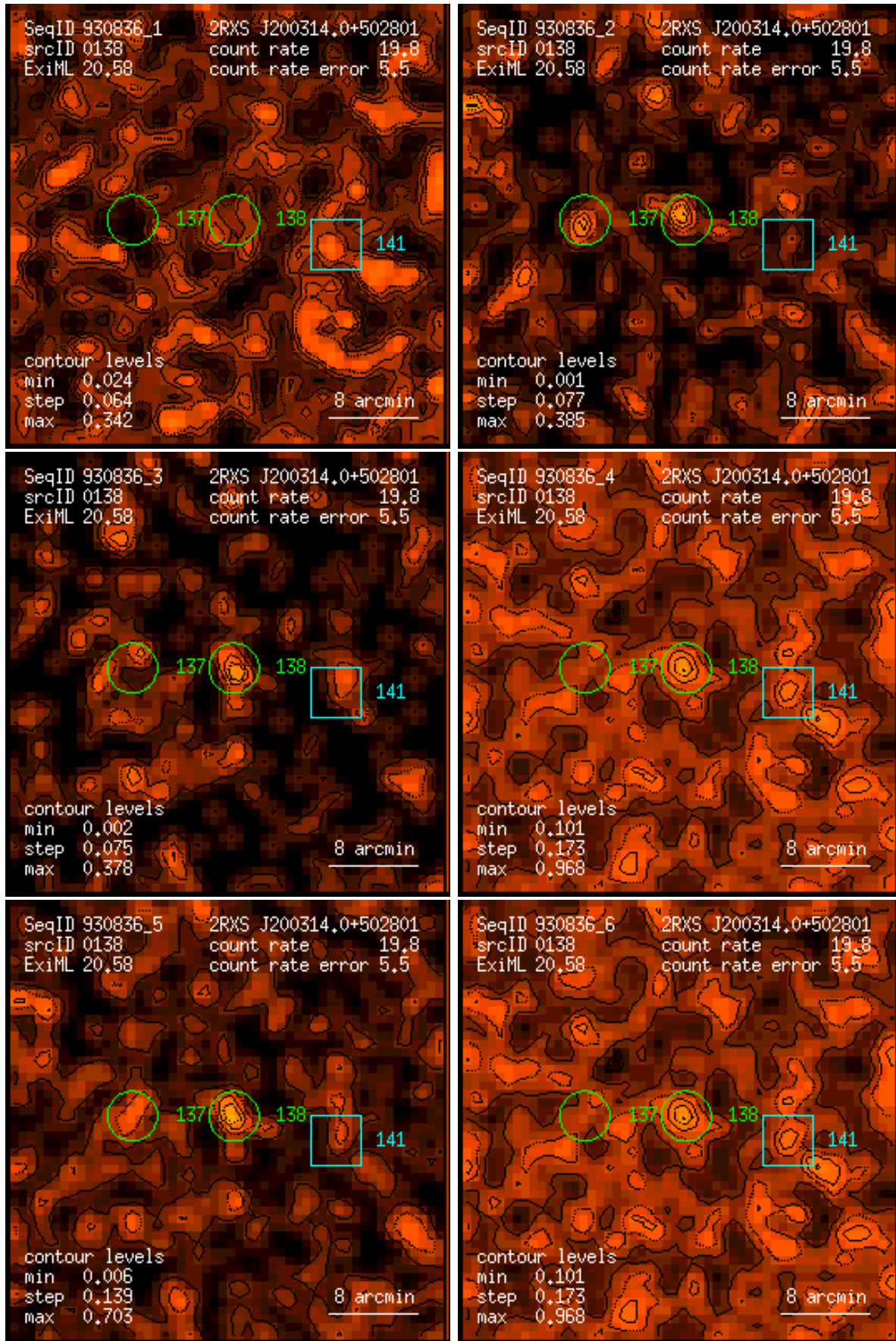
Figure 138: RASS 930836: detection 0138: band rate images, Gaussian filter: (1) PSPC channels 11 – 41, (2) 52 – 90, (3) 91 – 201, (4) 11 – 235, (5) 52 – 201, (6) 11 – 201. Broad band rates in counts/ks. Band rate contour levels in counts/ks/arcmin 2 .
