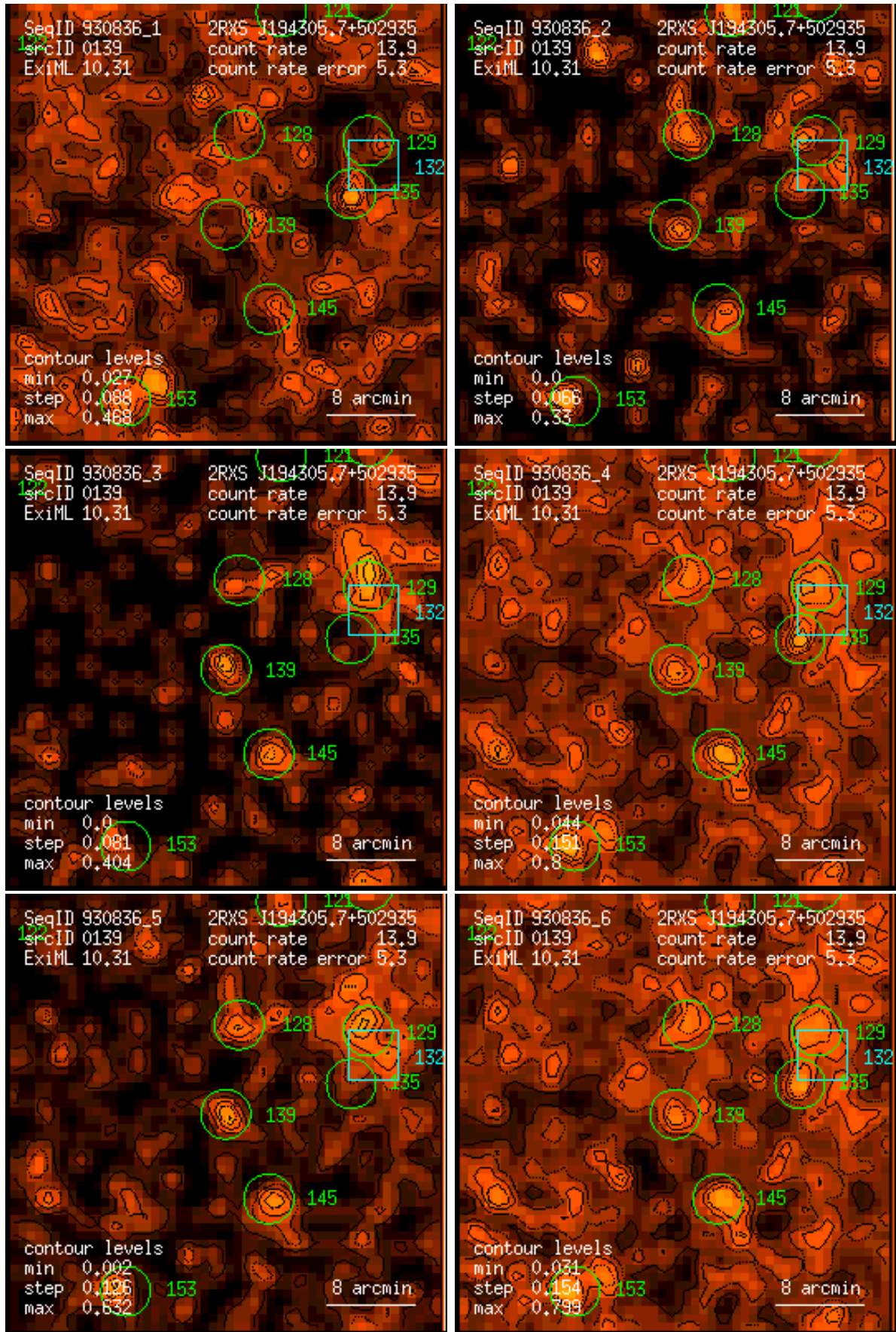
Figure 139: RASS 930836: detection 0139: band rate images, Gaussian filter: (1) PSPC channels 11 – 41, (2) 52 – 90, (3) 91 – 201, (4) 11 – 235, (5) 52 – 201, (6) 11 – 201. Broad band rates in counts/ks. Band rate contour levels in counts/ks/arcmin 2 .
