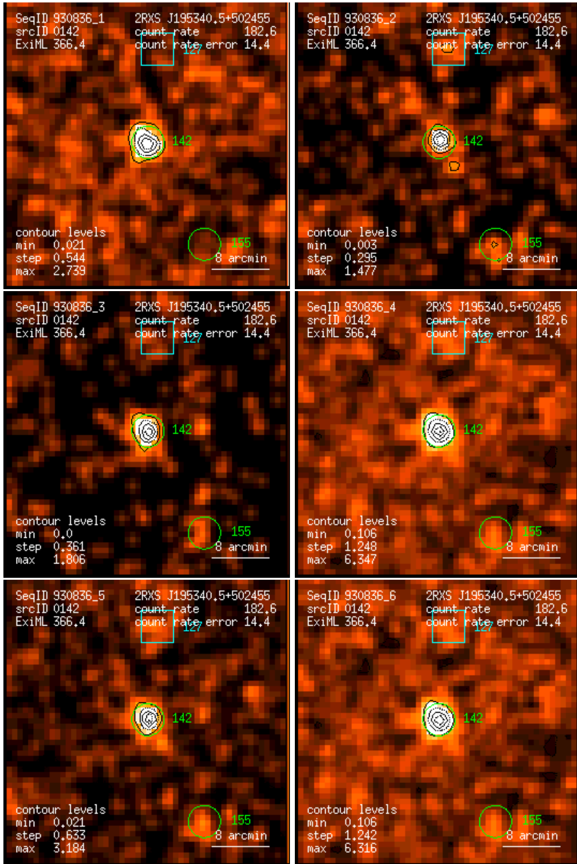
Figure 142: RASS 930836: detection 0142: band rate images, Gaussian filter: (1) PSPC channels 11 – 41, (2) 52 – 90, (3) 91 – 201, (4) 11 – 235, (5) 52 – 201, (6) 11 – 201. Broad band rates in counts/ks. Band rate contour levels in counts/ks/arcmin 2 .
