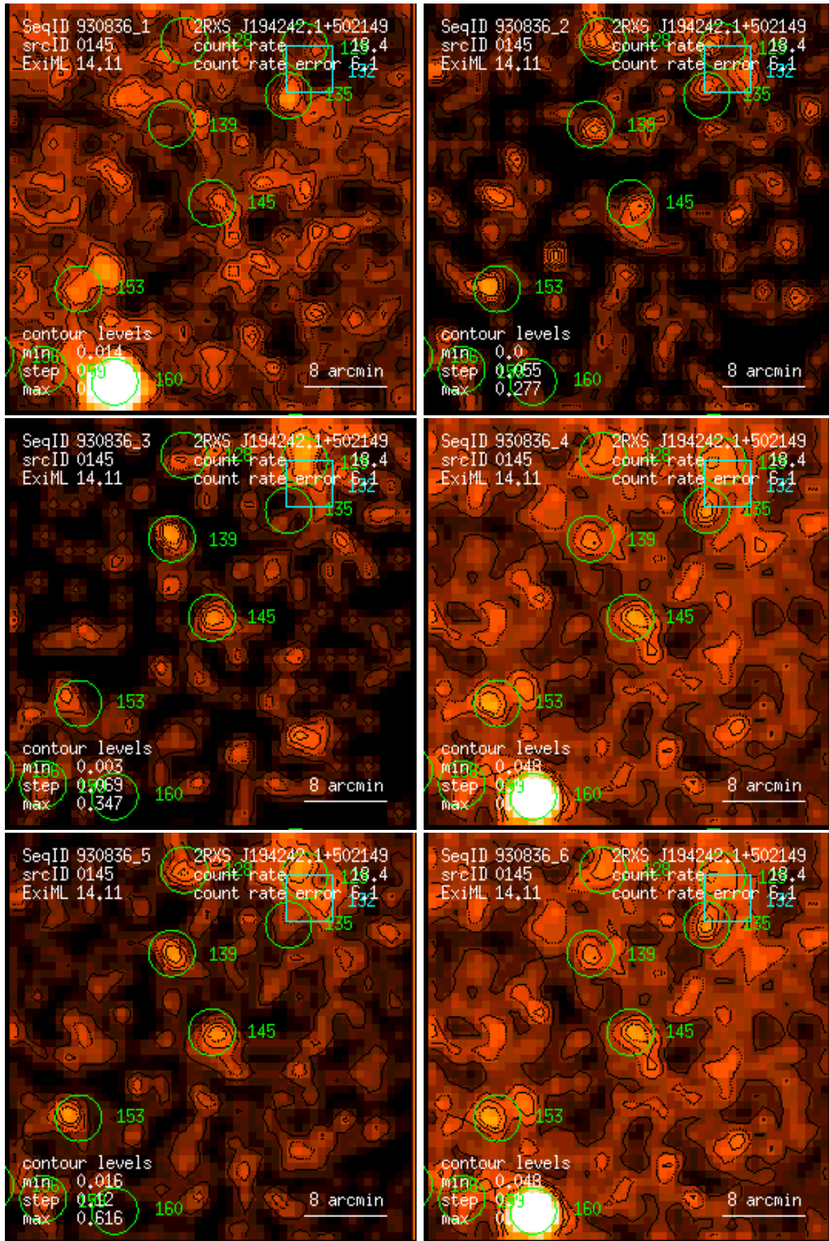
Figure 145: RASS 930836: detection 0145: band rate images, Gaussian filter: (1) PSPC channels 11 – 41, (2) 52 – 90, (3) 91 – 201, (4) 11 – 235, (5) 52 – 201, (6) 11 – 201. Broad band rates in counts/ks. Band rate contour levels in counts/ks/arcmin 2 .
