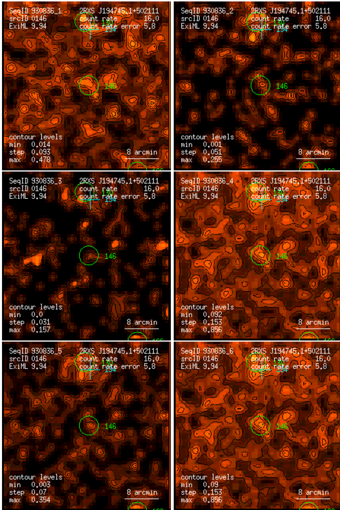
Figure 146: RASS 930836: detection 0146: band rate images, Gaussian filter: (1) PSPC channels 11 – 41, (2) 52 – 90, (3) 91 – 201, (4) 11 – 235, (5) 52 – 201, (6) 11 – 201. Broad band rates in counts/ks. Band rate contour levels in counts/ks/arcmin 2 .
