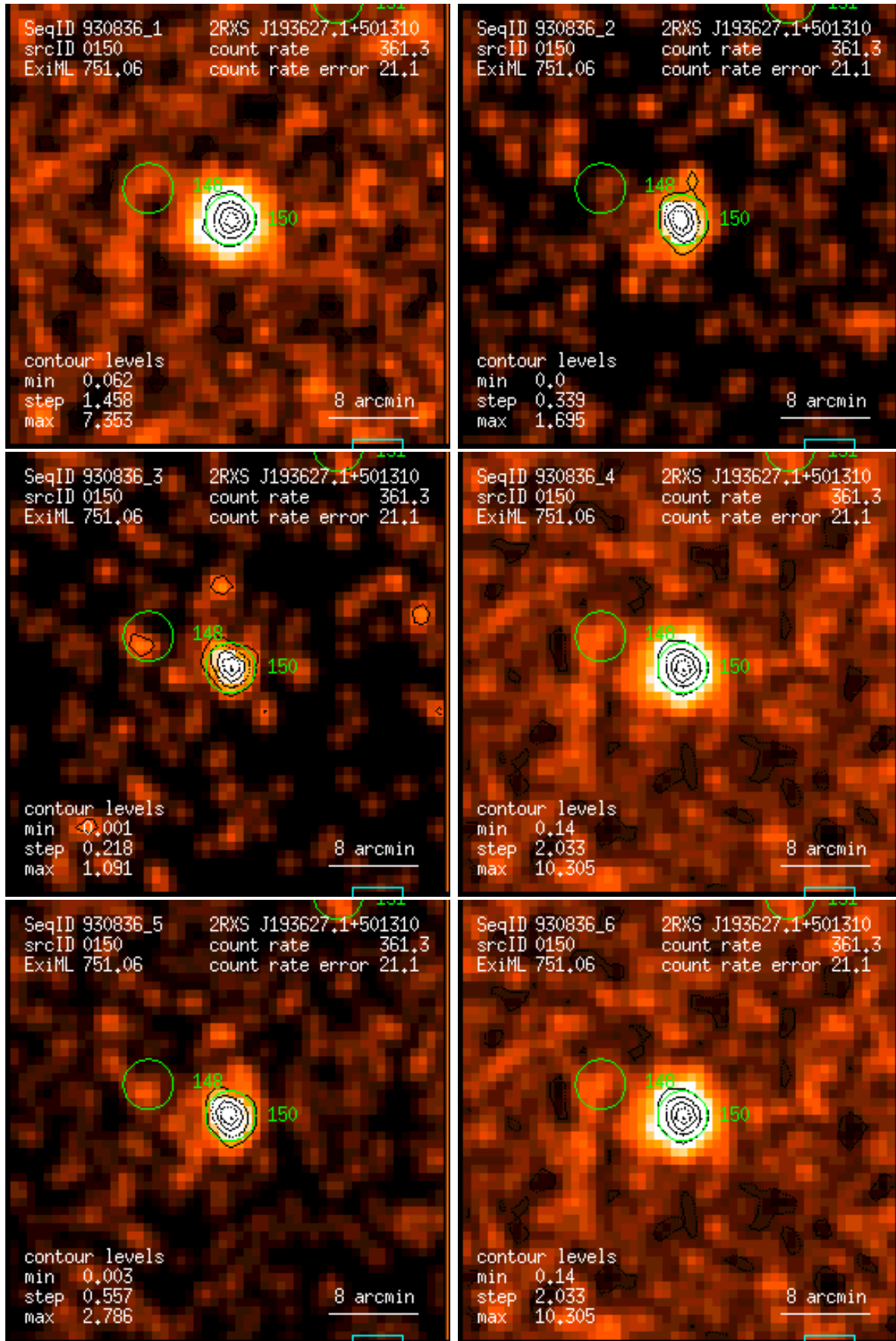
Figure 150: RASS 930836: detection 0150: band rate images, Gaussian filter: (1) PSPC channels 11 – 41, (2) 52 – 90, (3) 91 – 201, (4) 11 – 235, (5) 52 – 201, (6) 11 – 201. Broad band rates in counts/ks. Band rate contour levels in counts/ks/arcmin 2 .
