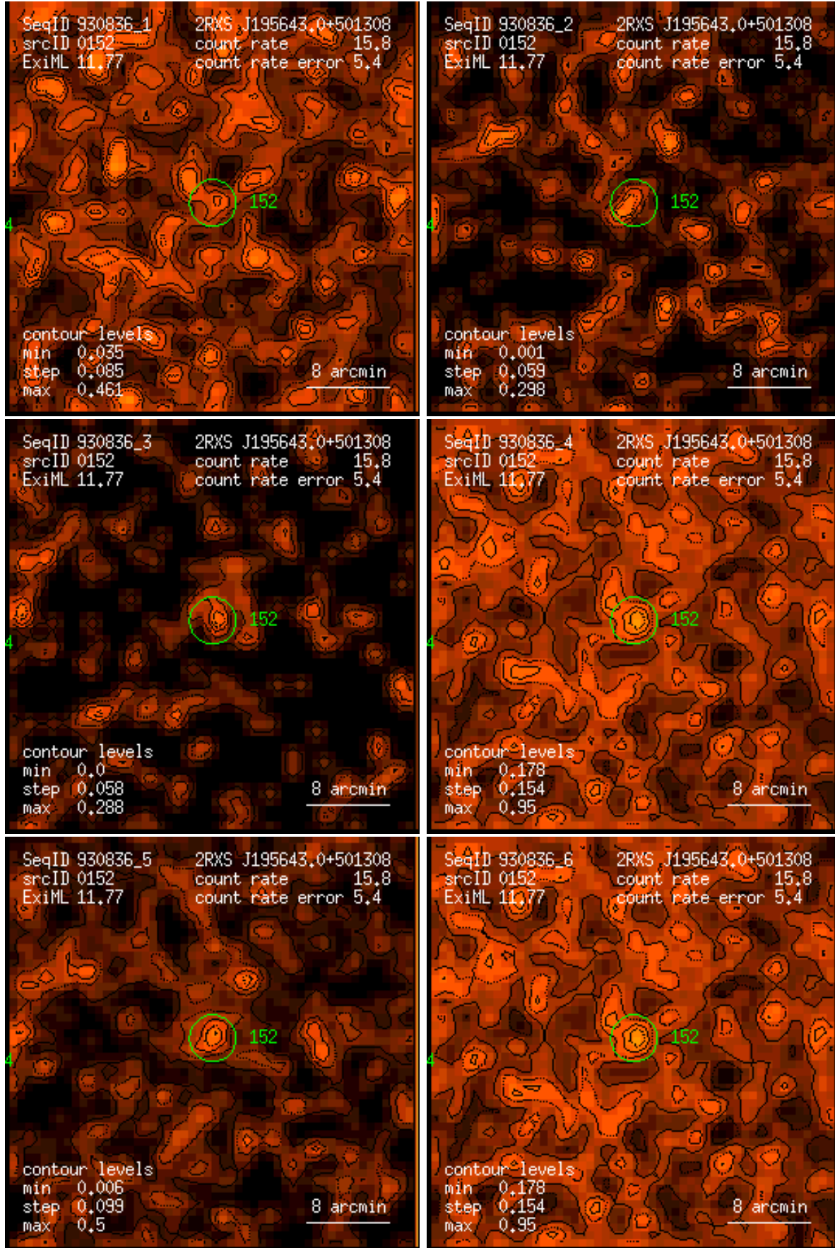
Figure 152: RASS 930836: detection 0152: band rate images, Gaussian filter: (1) PSPC channels 11 – 41, (2) 52 – 90, (3) 91 – 201, (4) 11 – 235, (5) 52 – 201, (6) 11 – 201. Broad band rates in counts/ks. Band rate contour levels in counts/ks/arcmin 2 .
