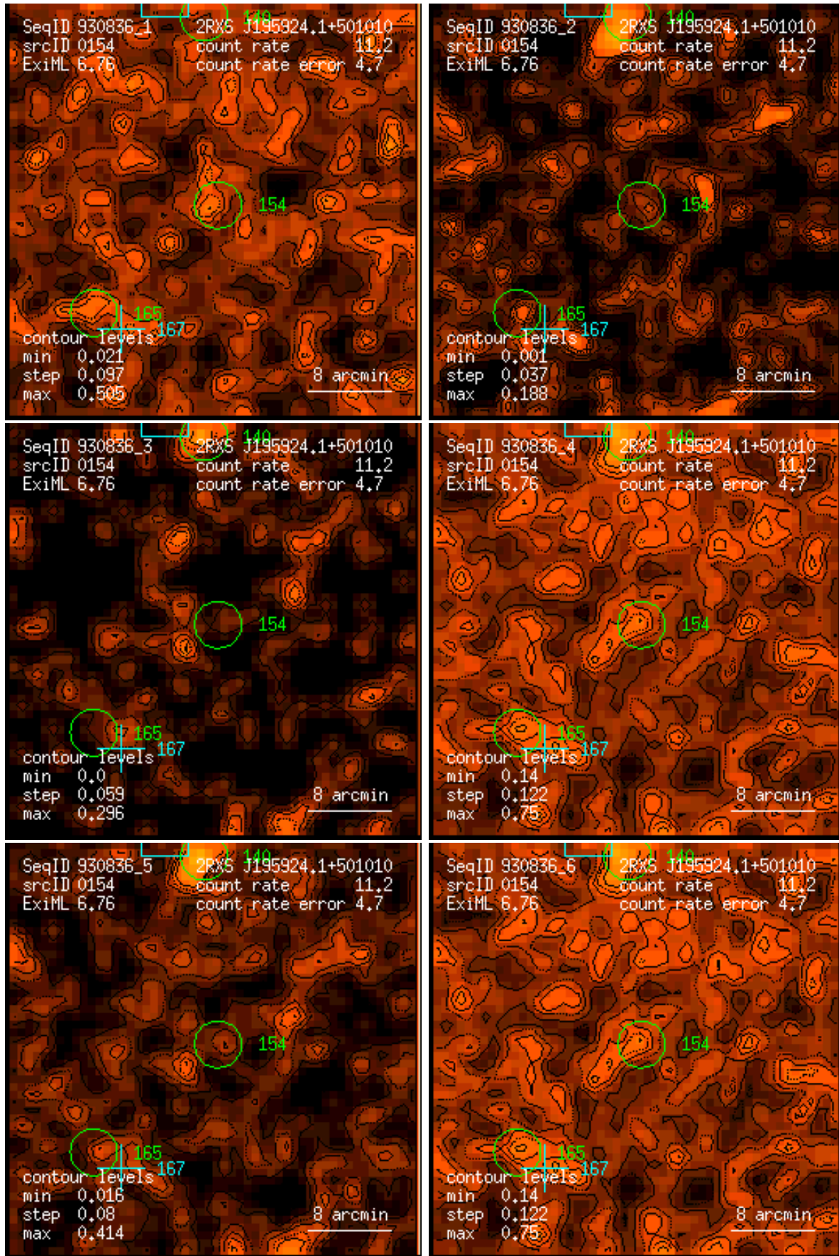
Figure 154: RASS 930836: detection 0154: band rate images, Gaussian filter: (1) PSPC channels 11 – 41, (2) 52 – 90, (3) 91 – 201, (4) 11 – 235, (5) 52 – 201, (6) 11 – 201. Broad band rates in counts/ks. Band rate contour levels in counts/ks/arcmin 2 .
