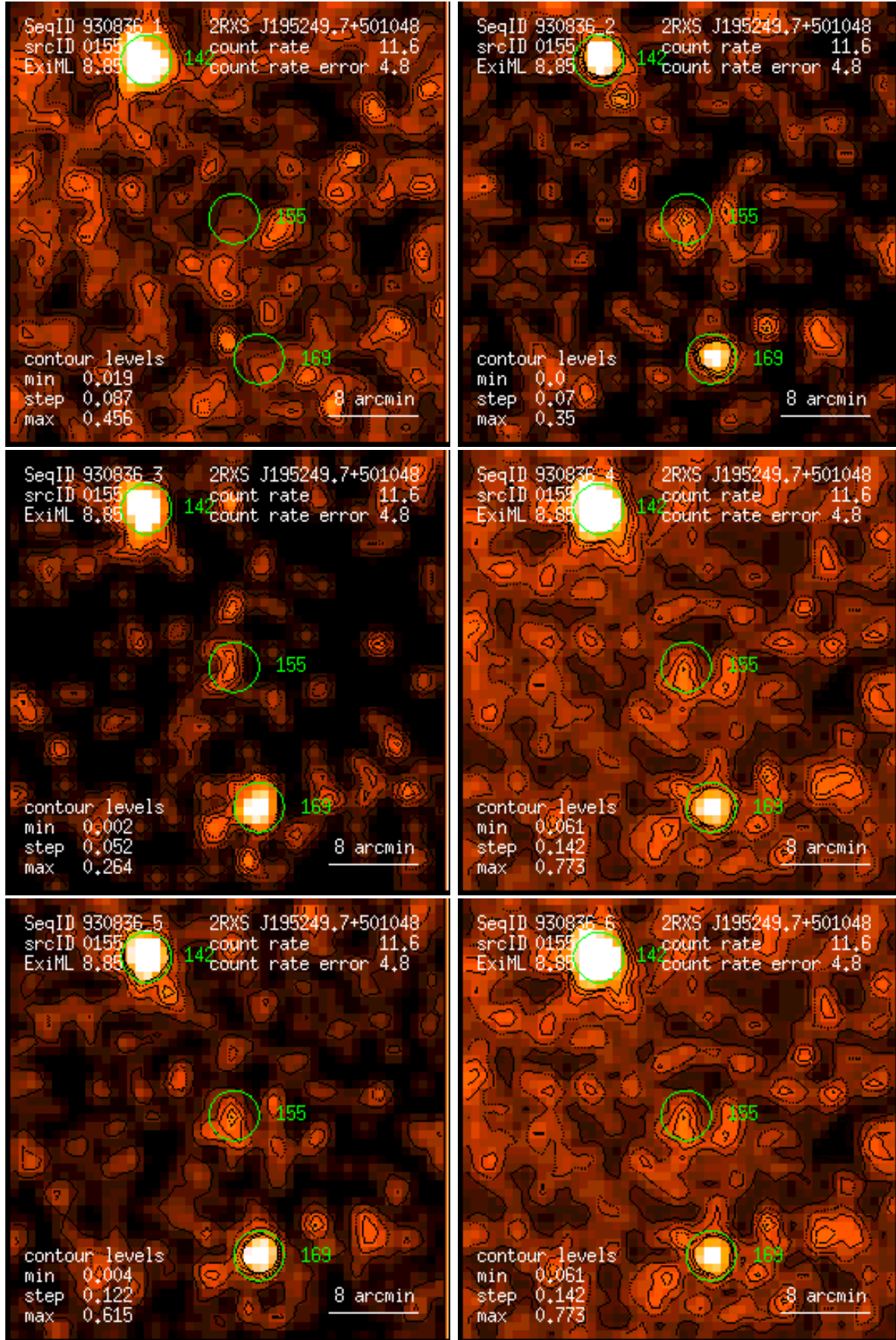
Figure 155: RASS 930836: detection 0155: band rate images, Gaussian filter: (1) PSPC channels 11 – 41, (2) 52 – 90, (3) 91 – 201, (4) 11 – 235, (5) 52 – 201, (6) 11 – 201. Broad band rates in counts/ks. Band rate contour levels in counts/ks/arcmin 2 .
