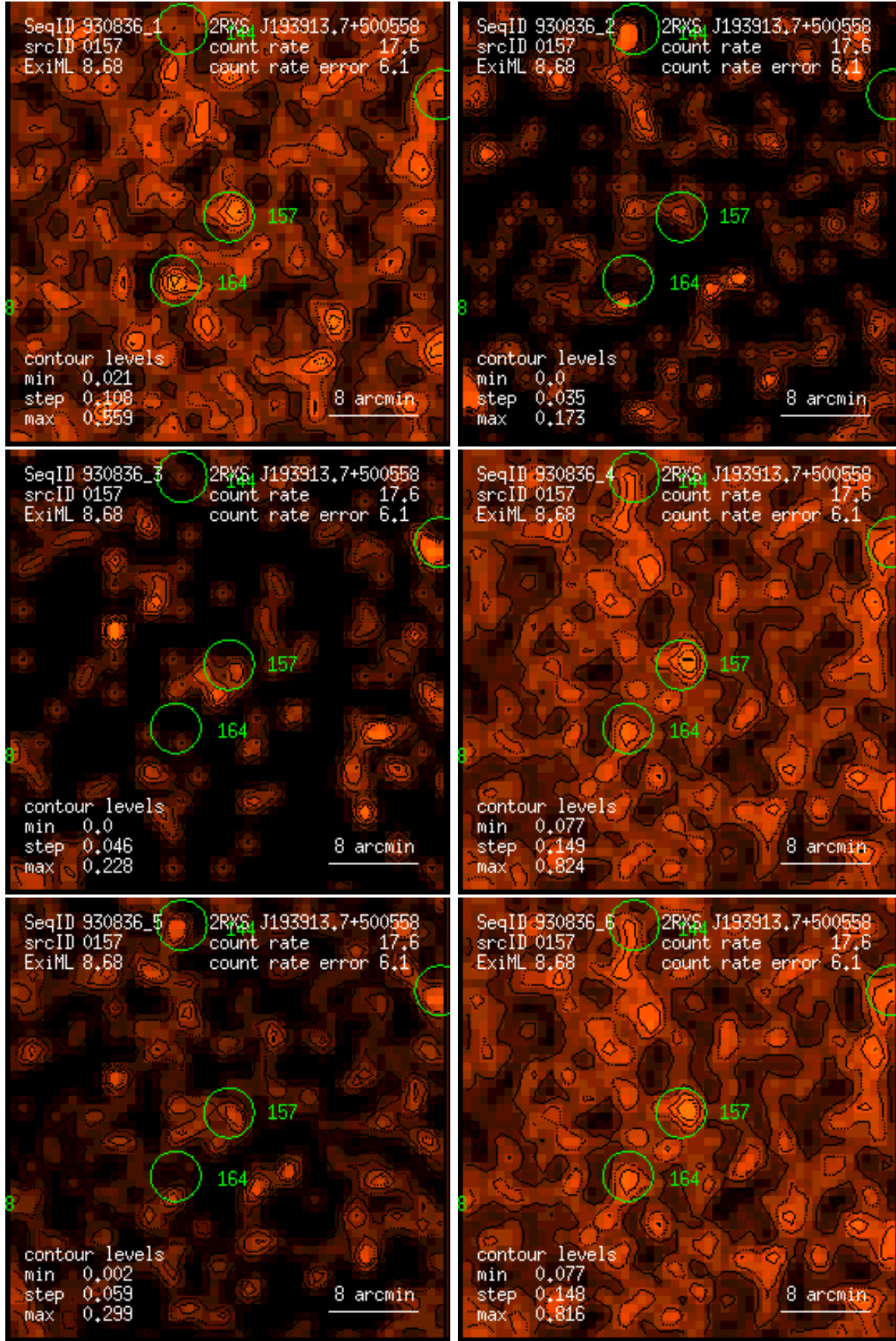
Figure 157: RASS 930836: detection 0157: band rate images, Gaussian filter: (1) PSPC channels 11 – 41, (2) 52 – 90, (3) 91 – 201, (4) 11 – 235, (5) 52 – 201, (6) 11 – 201. Broad band rates in counts/ks. Band rate contour levels in counts/ks/arcmin 2 .
