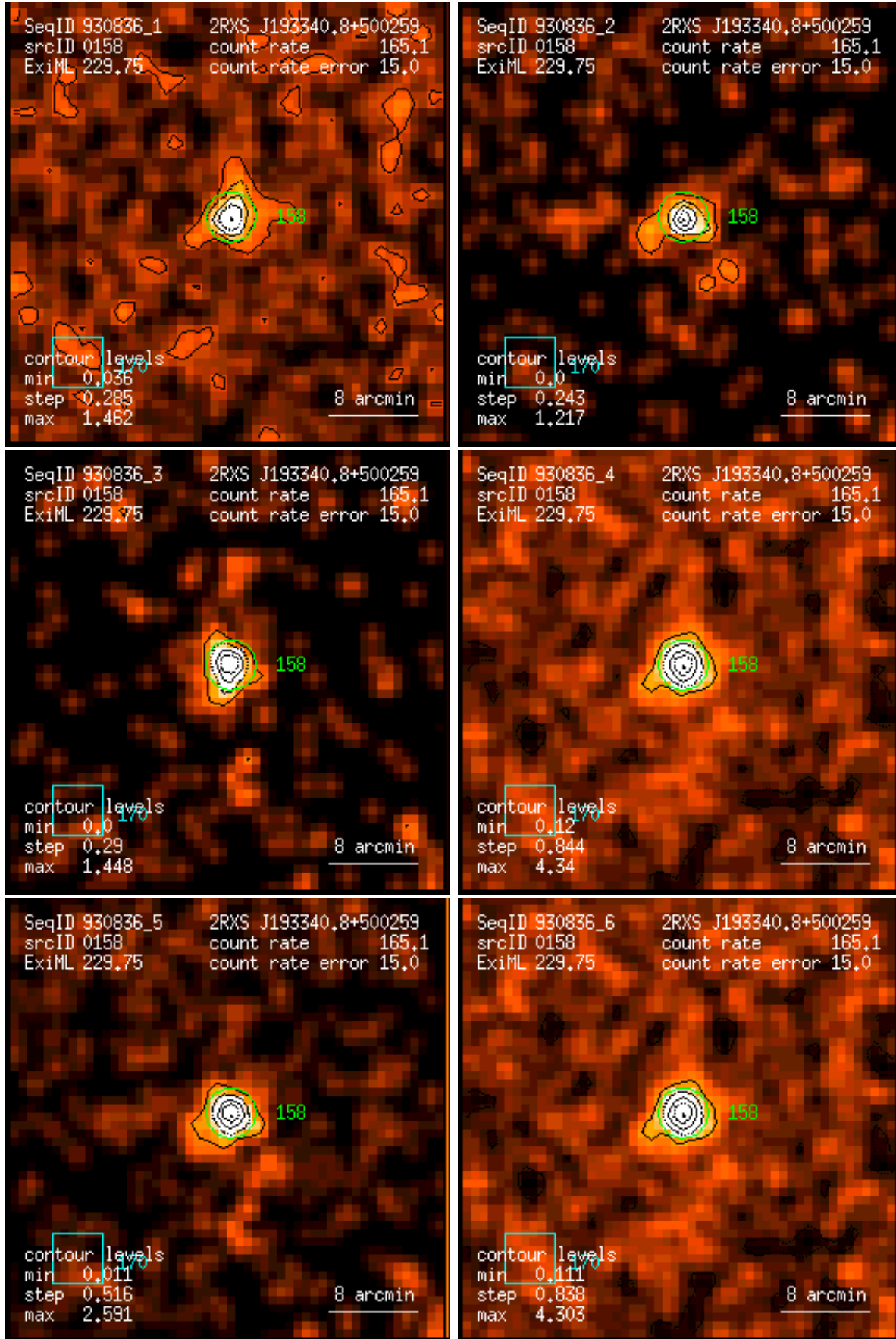
Figure 158: RASS 930836: detection 0158: band rate images, Gaussian filter: (1) PSPC channels 11 – 41, (2) 52 – 90, (3) 91 – 201, (4) 11 – 235, (5) 52 – 201, (6) 11 – 201. Broad band rates in counts/ks. Band rate contour levels in counts/ks/arcmin 2 .
