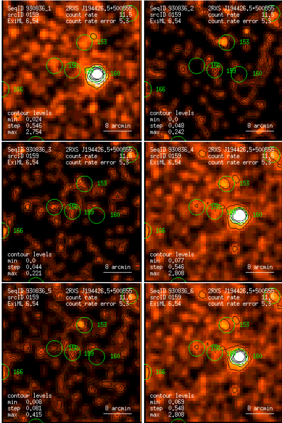
Figure 159: RASS 930836: detection 0159: band rate images, Gaussian filter: (1) PSPC channels 11 – 41, (2) 52 – 90, (3) 91 – 201, (4) 11 – 235, (5) 52 – 201, (6) 11 – 201. Broad band rates in counts/ks. Band rate contour levels in counts/ks/arcmin 2 .
