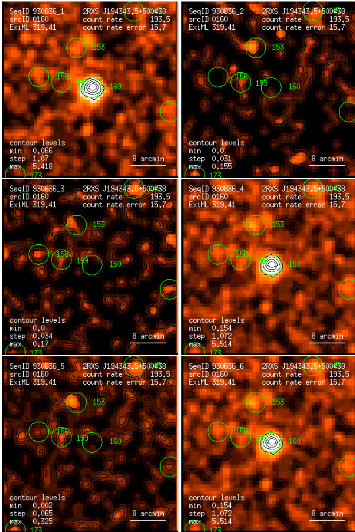
Figure 160: RASS 930836: detection 0160: band rate images, Gaussian filter: (1) PSPC channels 11 – 41, (2) 52 – 90, (3) 91 – 201, (4) 11 – 235, (5) 52 – 201, (6) 11 – 201. Broad band rates in counts/ks. Band rate contour levels in counts/ks/arcmin 2 .
