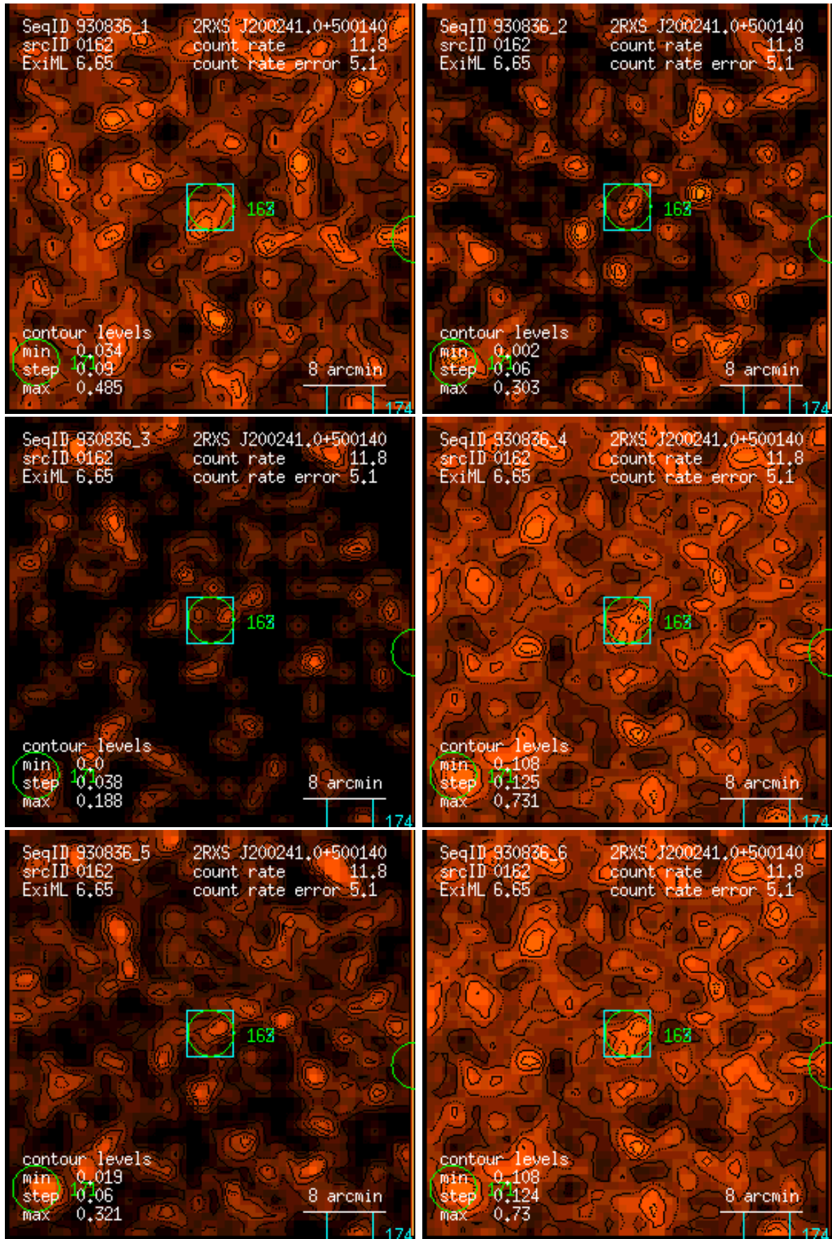
Figure 162: RASS 930836: detection 0162: band rate images, Gaussian filter: (1) PSPC channels 11 – 41, (2) 52 – 90, (3) 91 – 201, (4) 11 – 235, (5) 52 – 201, (6) 11 – 201. Broad band rates in counts/ks. Band rate contour levels in counts/ks/arcmin 2 .
