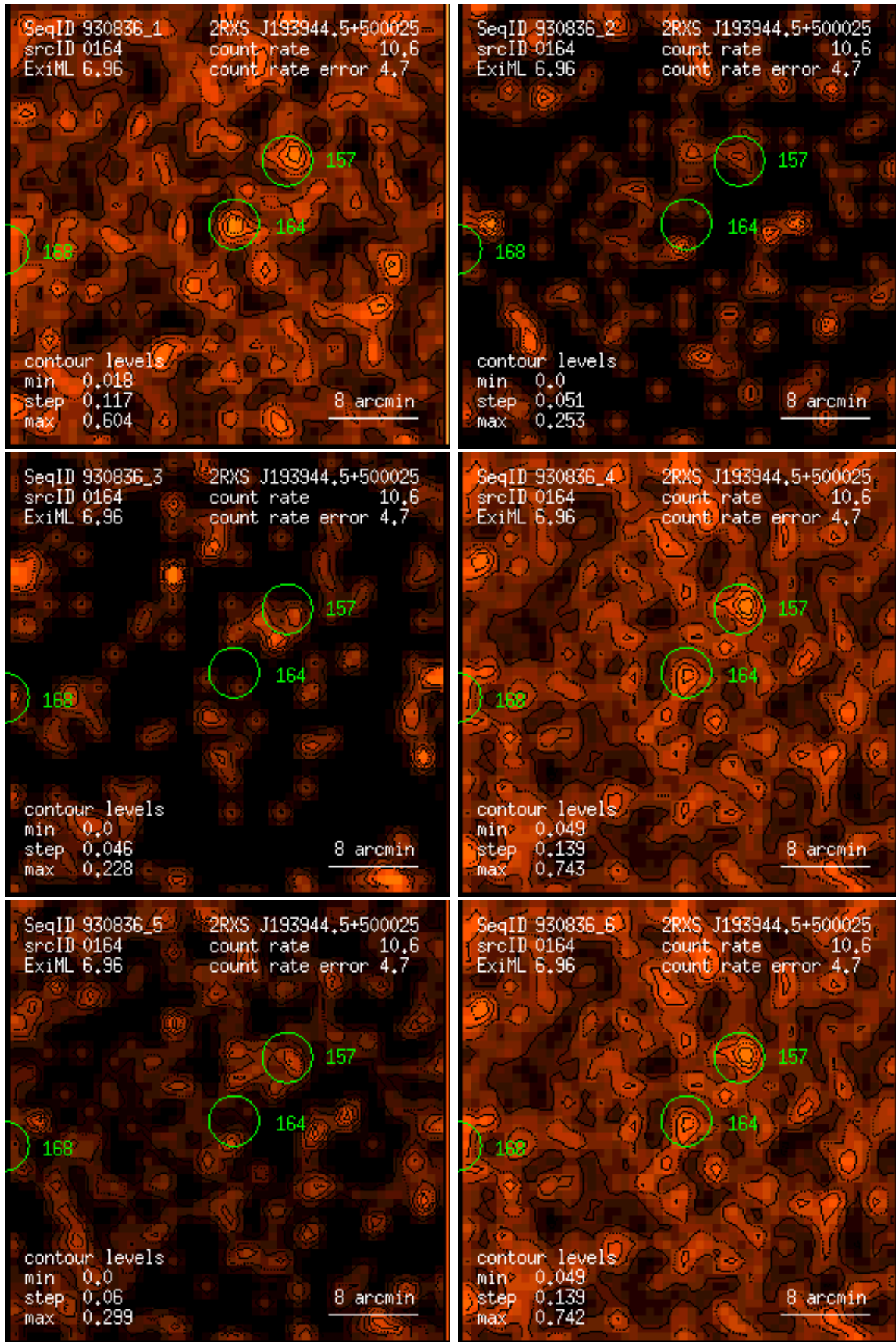
Figure 164: RASS 930836: detection 0164: band rate images, Gaussian filter: (1) PSPC channels 11 – 41, (2) 52 – 90, (3) 91 – 201, (4) 11 – 235, (5) 52 – 201, (6) 11 – 201. Broad band rates in counts/ks. Band rate contour levels in counts/ks/arcmin 2 .
