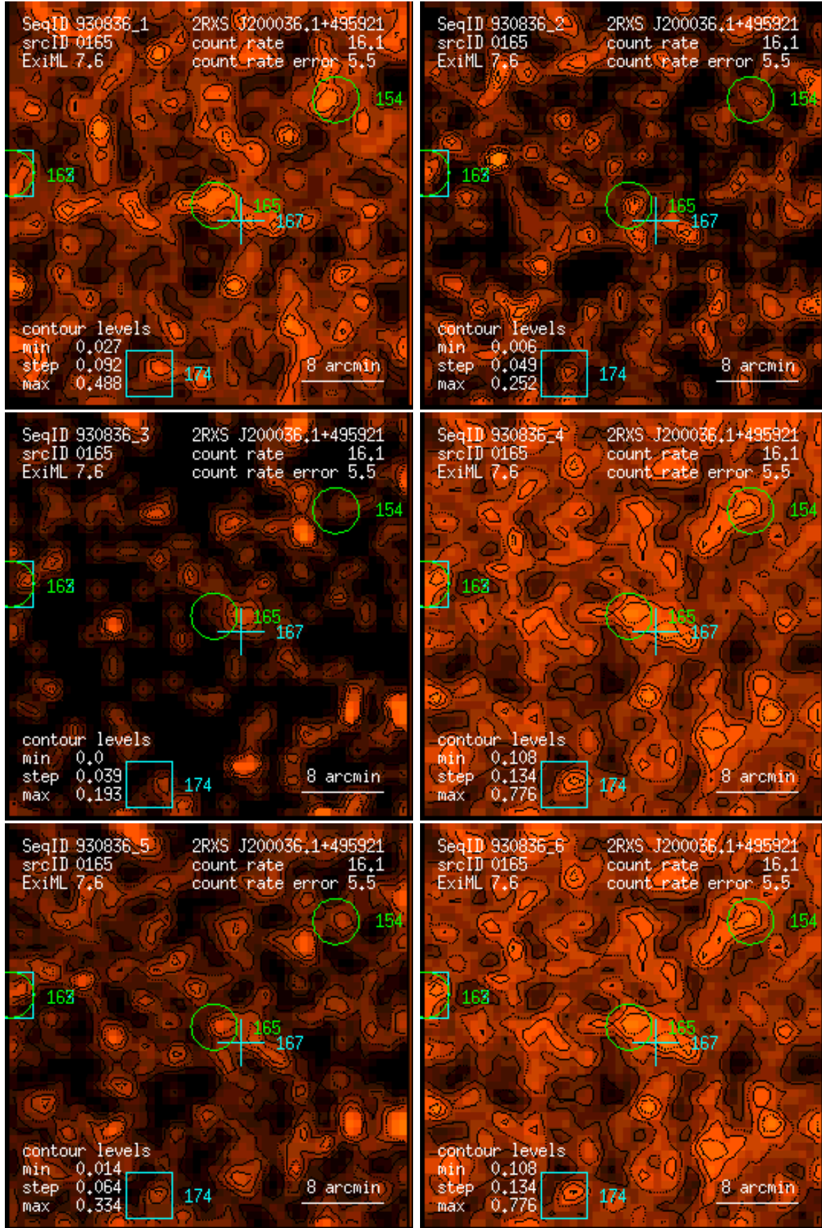
Figure 165: RASS 930836: detection 0165: band rate images, Gaussian filter: (1) PSPC channels 11 – 41, (2) 52 – 90, (3) 91 – 201, (4) 11 – 235, (5) 52 – 201, (6) 11 – 201. Broad band rates in counts/ks. Band rate contour levels in counts/ks/arcmin 2 .
