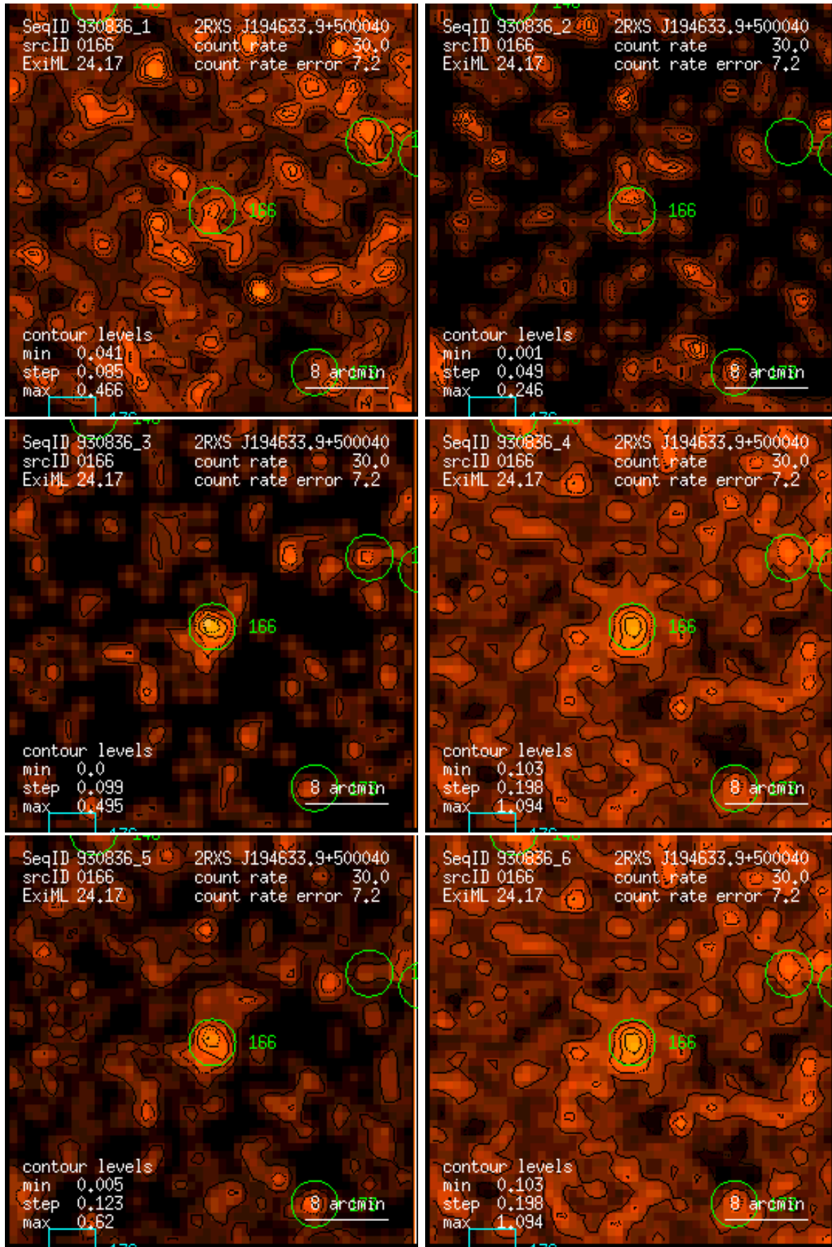
Figure 166: RASS 930836: detection 0166: band rate images, Gaussian filter: (1) PSPC channels 11 – 41, (2) 52 – 90, (3) 91 – 201, (4) 11 – 235, (5) 52 – 201, (6) 11 – 201. Broad band rates in counts/ks. Band rate contour levels in counts/ks/arcmin 2 .
