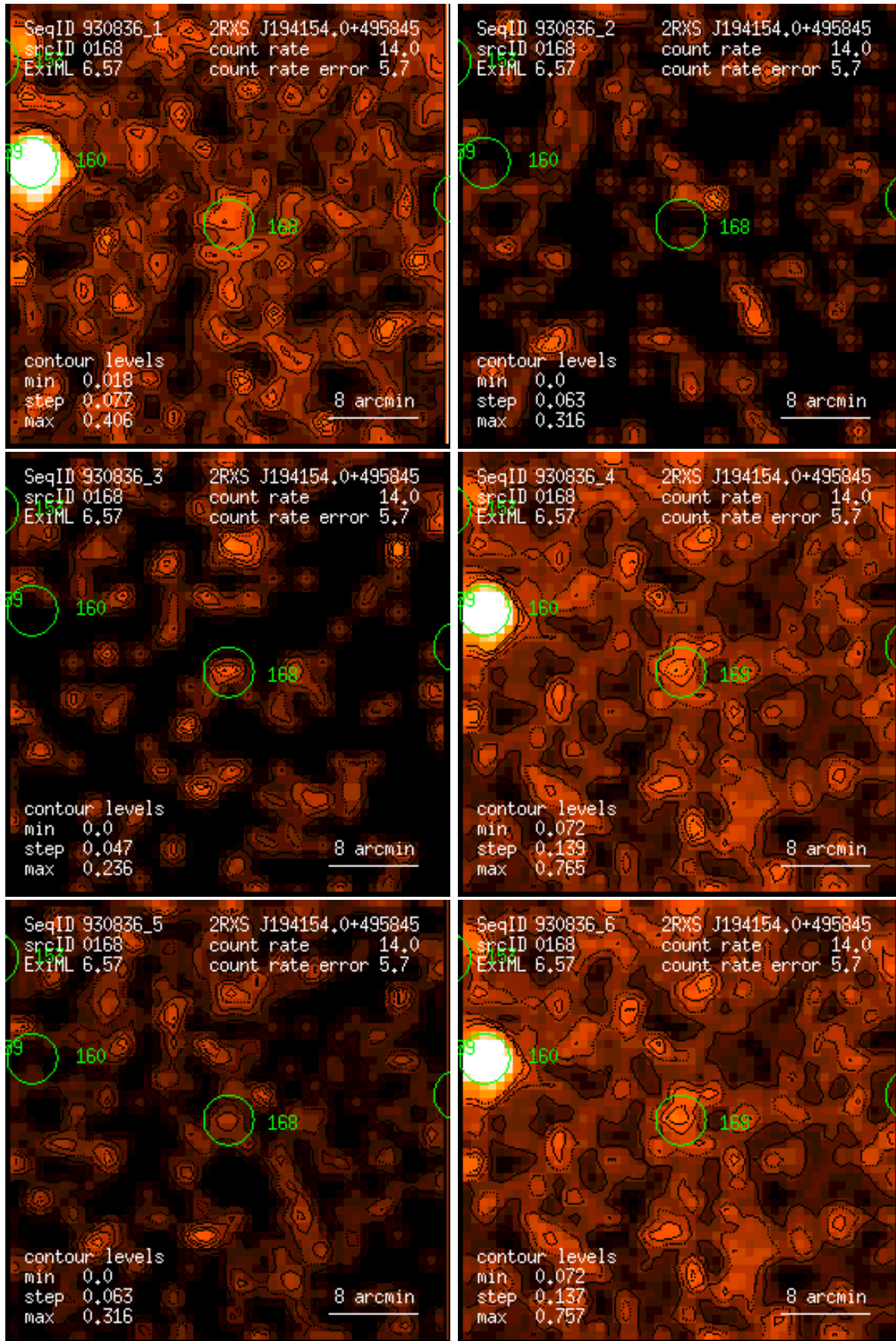
Figure 168: RASS 930836: detection 0168: band rate images, Gaussian filter: (1) PSPC channels 11 – 41, (2) 52 – 90, (3) 91 – 201, (4) 11 – 235, (5) 52 – 201, (6) 11 – 201. Broad band rates in counts/ks. Band rate contour levels in counts/ks/arcmin 2 .
