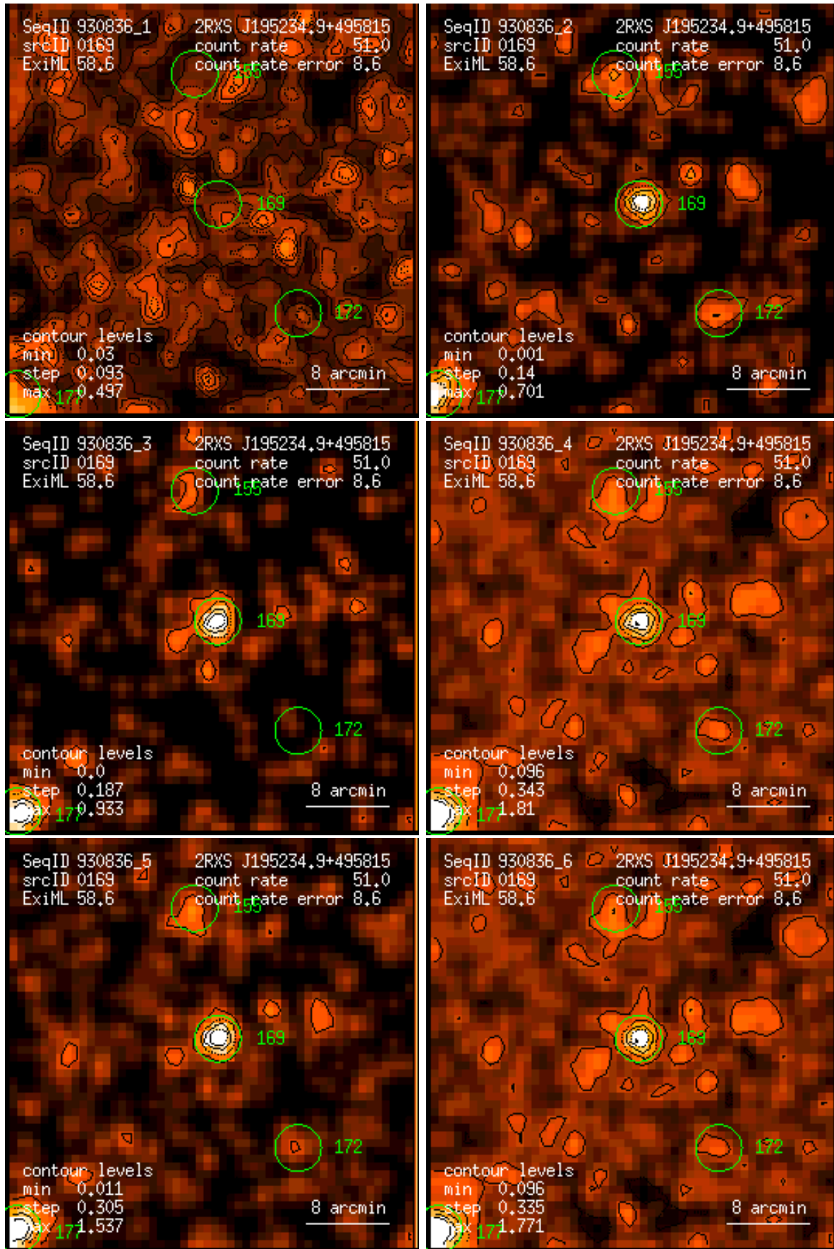
Figure 169: RASS 930836: detection 0169: band rate images, Gaussian filter: (1) PSPC channels 11 – 41, (2) 52 – 90, (3) 91 – 201, (4) 11 – 235, (5) 52 – 201, (6) 11 – 201. Broad band rates in counts/ks. Band rate contour levels in counts/ks/arcmin 2 .
