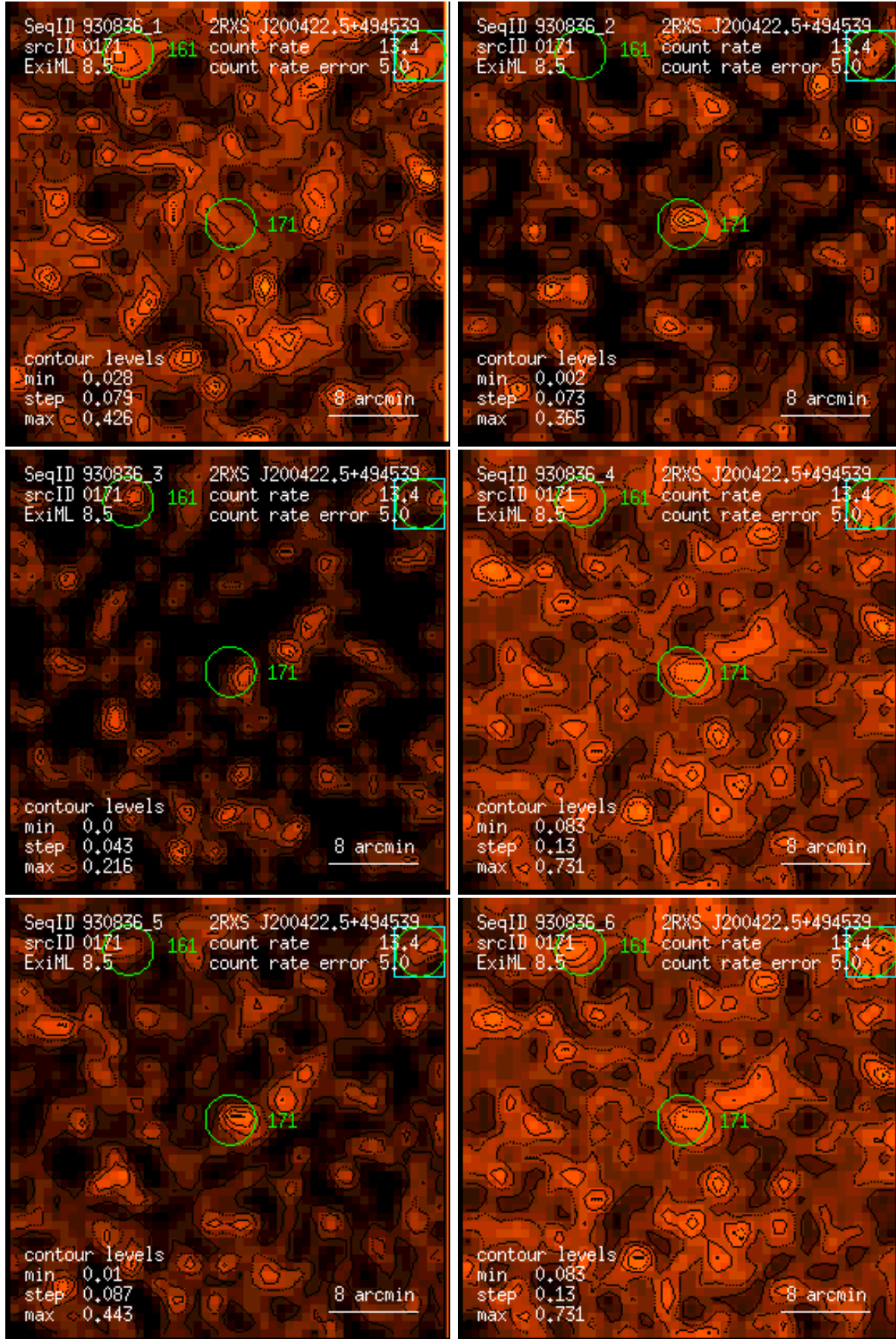
Figure 171: RASS 930836: detection 0171: band rate images, Gaussian filter: (1) PSPC channels 11 – 41, (2) 52 – 90, (3) 91 – 201, (4) 11 – 235, (5) 52 – 201, (6) 11 – 201. Broad band rates in counts/ks. Band rate contour levels in counts/ks/arcmin 2 .
