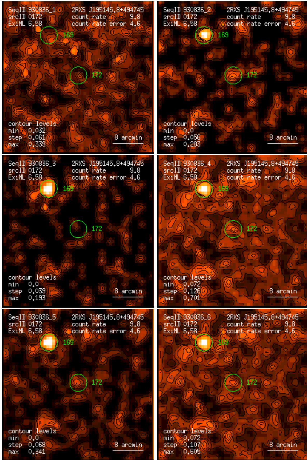
Figure 172: RASS 930836: detection 0172: band rate images, Gaussian filter: (1) PSPC channels 11 – 41, (2) 52 – 90, (3) 91 – 201, (4) 11 – 235, (5) 52 – 201, (6) 11 – 201. Broad band rates in counts/ks. Band rate contour levels in counts/ks/arcmin 2 .
