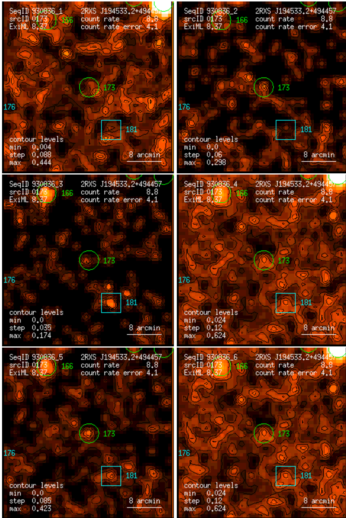
Figure 173: RASS 930836: detection 0173: band rate images, Gaussian filter: (1) PSPC channels 11 – 41, (2) 52 – 90, (3) 91 – 201, (4) 11 – 235, (5) 52 – 201, (6) 11 – 201. Broad band rates in counts/ks. Band rate contour levels in counts/ks/arcmin 2 .
