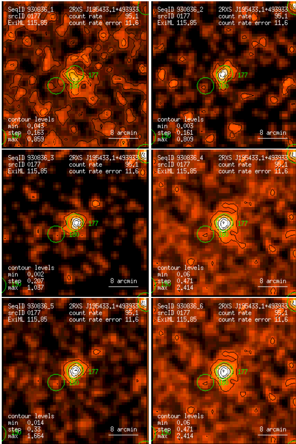
Figure 177: RASS 930836: detection 0177: band rate images, Gaussian filter: (1) PSPC channels 11 – 41, (2) 52 – 90, (3) 91 – 201, (4) 11 – 235, (5) 52 – 201, (6) 11 – 201. Broad band rates in counts/ks. Band rate contour levels in counts/ks/arcmin 2 .
