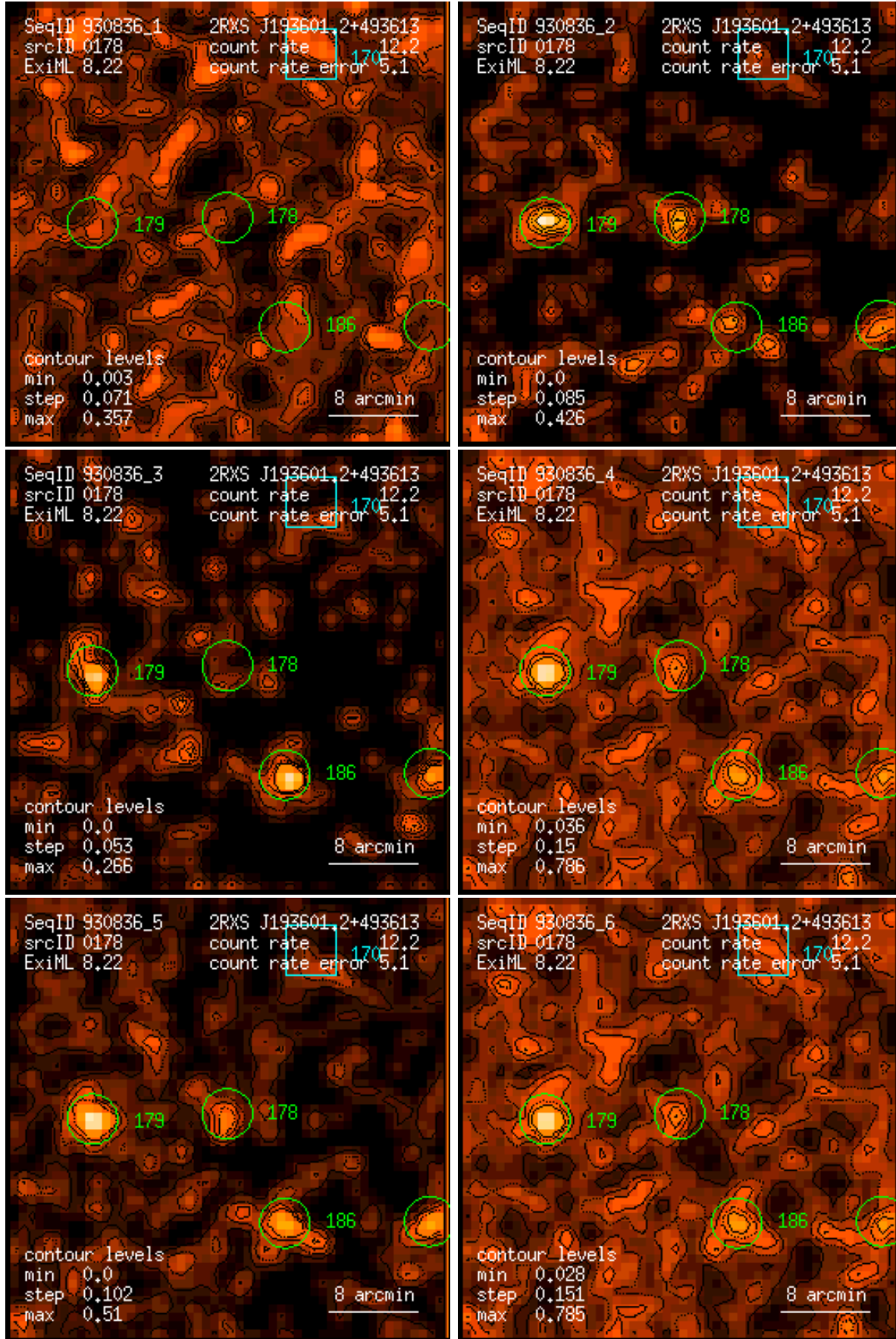
Figure 178: RASS 930836: detection 0178: band rate images, Gaussian filter: (1) PSPC channels 11 – 41, (2) 52 – 90, (3) 91 – 201, (4) 11 – 235, (5) 52 – 201, (6) 11 – 201. Broad band rates in counts/ks. Band rate contour levels in counts/ks/arcmin 2 .
