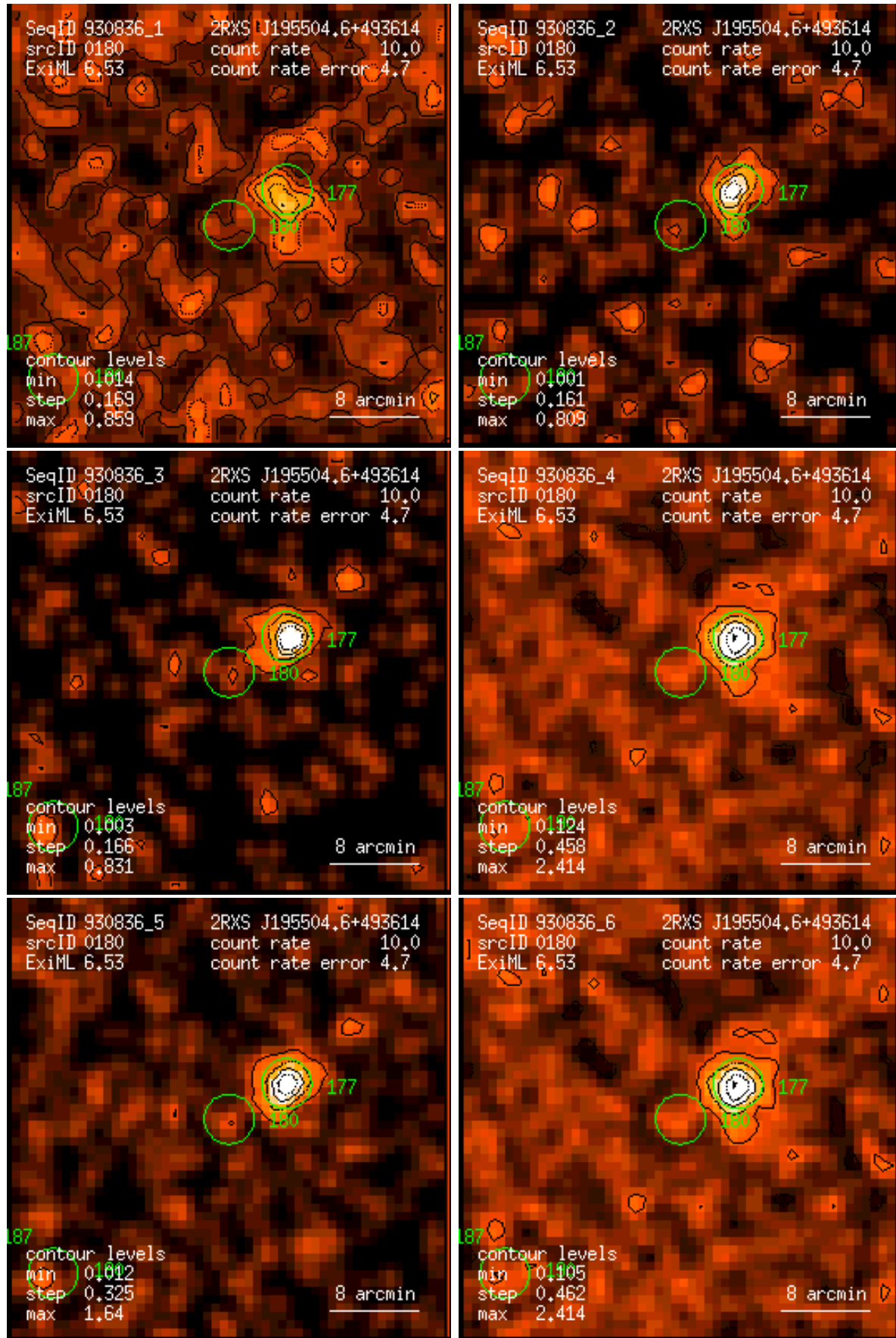
Figure 180: RASS 930836: detection 0180: band rate images, Gaussian filter: (1) PSPC channels 11 – 41, (2) 52 – 90, (3) 91 – 201, (4) 11 – 235, (5) 52 – 201, (6) 11 – 201. Broad band rates in counts/ks. Band rate contour levels in counts/ks/arcmin 2 .
