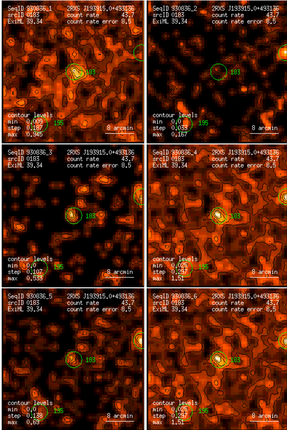
Figure 183: RASS 930836: detection 0183: band rate images, Gaussian filter: (1) PSPC channels 11 – 41, (2) 52 – 90, (3) 91 – 201, (4) 11 – 235, (5) 52 – 201, (6) 11 – 201. Broad band rates in counts/ks. Band rate contour levels in counts/ks/arcmin 2 .
