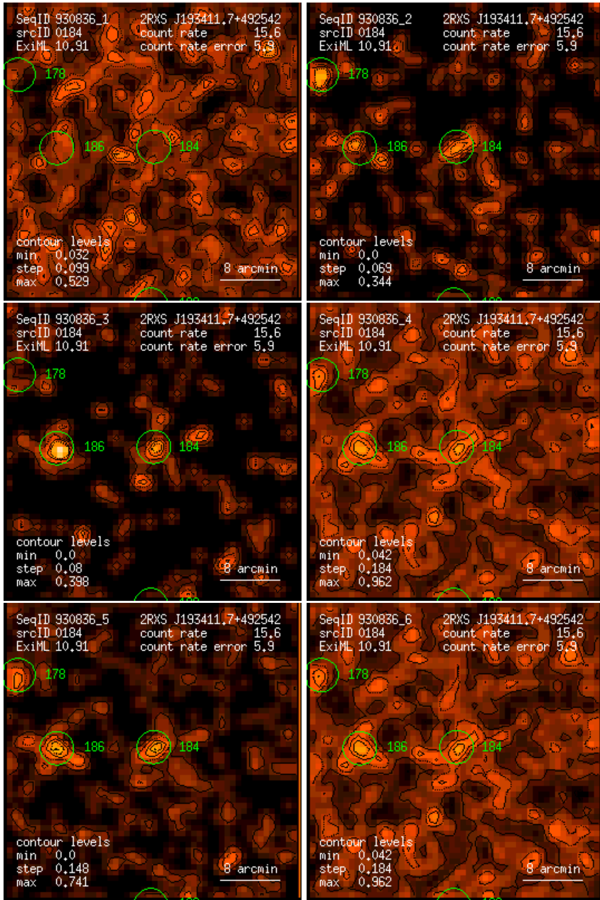
Figure 184: RASS 930836: detection 0184: band rate images, Gaussian filter: (1) PSPC channels 11 – 41, (2) 52 – 90, (3) 91 – 201, (4) 11 – 235, (5) 52 – 201, (6) 11 – 201. Broad band rates in counts/ks. Band rate contour levels in counts/ks/arcmin 2 .
