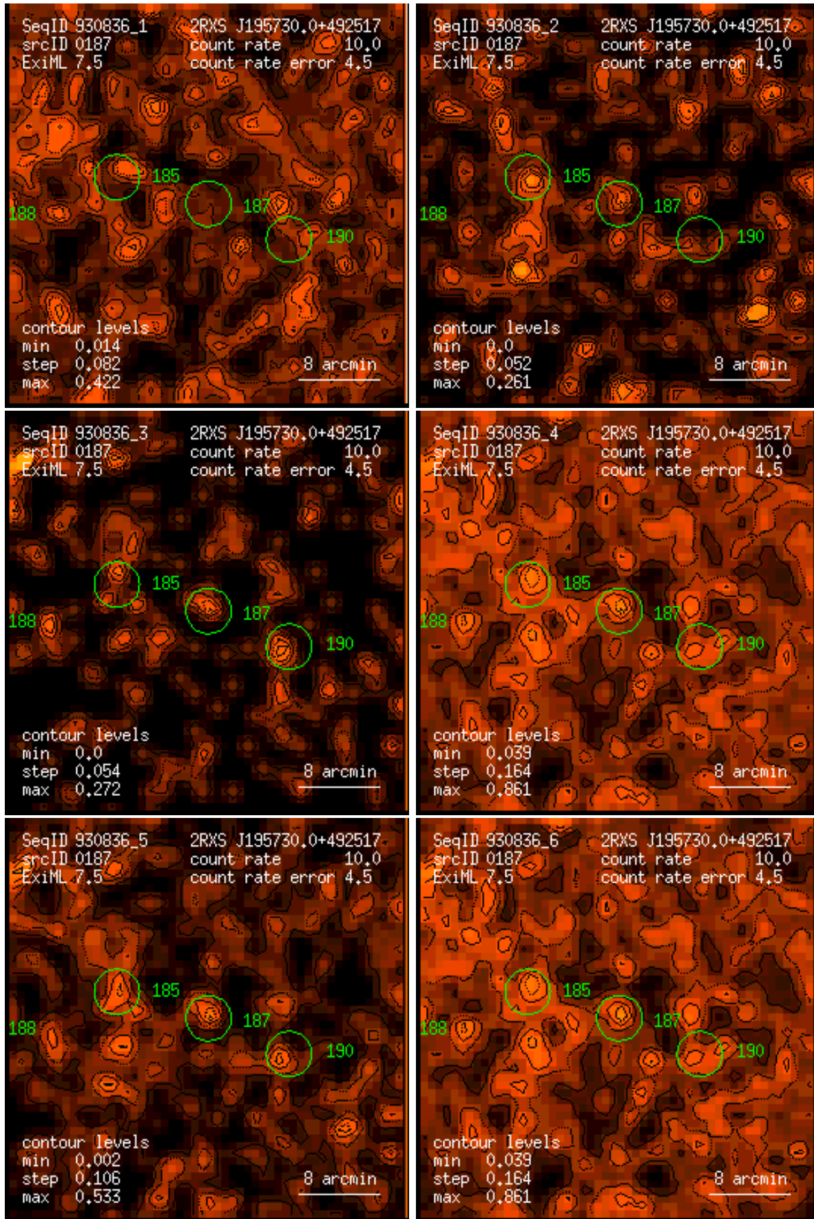
Figure 187: RASS 930836: detection 0187: band rate images, Gaussian filter: (1) PSPC channels 11 – 41, (2) 52 – 90, (3) 91 – 201, (4) 11 – 235, (5) 52 – 201, (6) 11 – 201. Broad band rates in counts/ks. Band rate contour levels in counts/ks/arcmin 2 .
