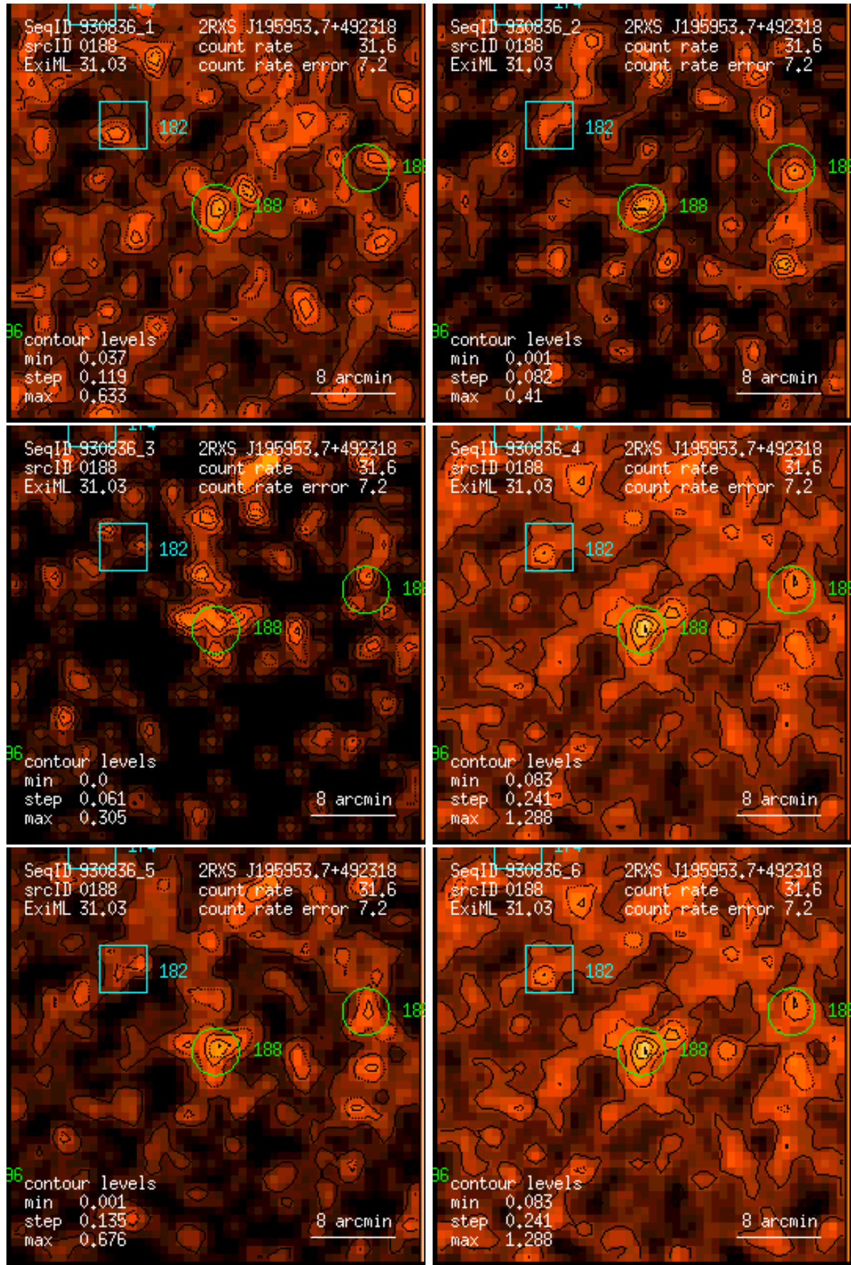
Figure 188: RASS 930836: detection 0188: band rate images, Gaussian filter: (1) PSPC channels 11 – 41, (2) 52 – 90, (3) 91 – 201, (4) 11 – 235, (5) 52 – 201, (6) 11 – 201. Broad band rates in counts/ks. Band rate contour levels in counts/ks/arcmin 2 .
