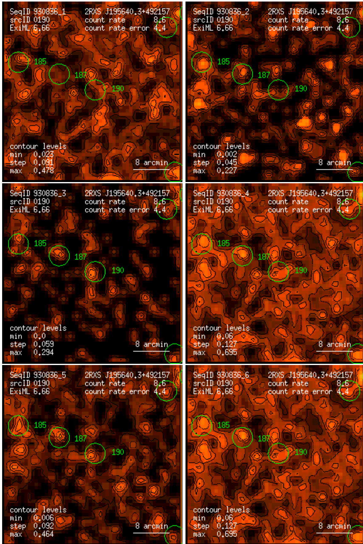
Figure 190: RASS 930836: detection 0190: band rate images, Gaussian filter: (1) PSPC channels 11 – 41, (2) 52 – 90, (3) 91 – 201, (4) 11 – 235, (5) 52 – 201, (6) 11 – 201. Broad band rates in counts/ks. Band rate contour levels in counts/ks/arcmin 2 .
