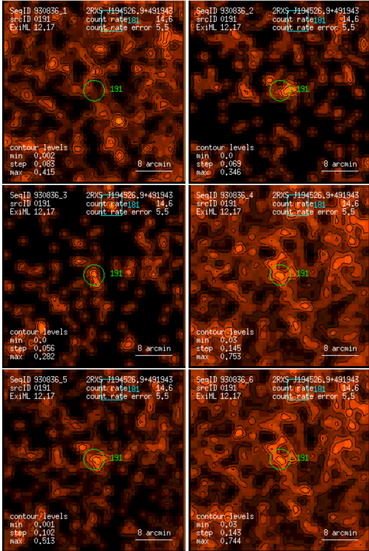
Figure 191: RASS 930836: detection 0191: band rate images, Gaussian filter: (1) PSPC channels 11 – 41, (2) 52 – 90, (3) 91 – 201, (4) 11 – 235, (5) 52 – 201, (6) 11 – 201. Broad band rates in counts/ks. Band rate contour levels in counts/ks/arcmin 2 .
