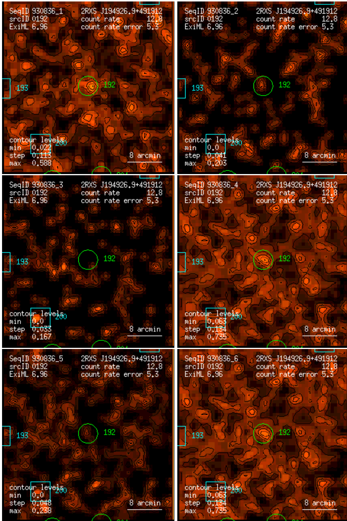
Figure 192: RASS 930836: detection 0192: band rate images, Gaussian filter: (1) PSPC channels 11 – 41, (2) 52 – 90, (3) 91 – 201, (4) 11 – 235, (5) 52 – 201, (6) 11 – 201. Broad band rates in counts/ks. Band rate contour levels in counts/ks/arcmin 2 .
