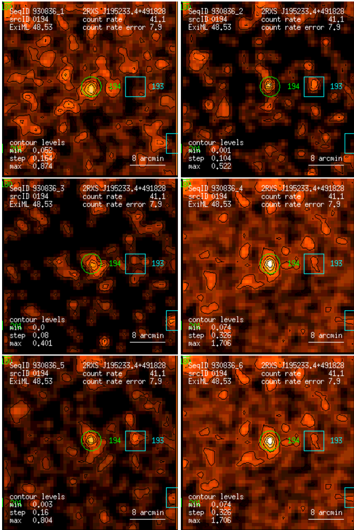
Figure 194: RASS 930836: detection 0194: band rate images, Gaussian filter: (1) PSPC channels 11 – 41, (2) 52 – 90, (3) 91 – 201, (4) 11 – 235, (5) 52 – 201, (6) 11 – 201. Broad band rates in counts/ks. Band rate contour levels in counts/ks/arcmin 2 .
