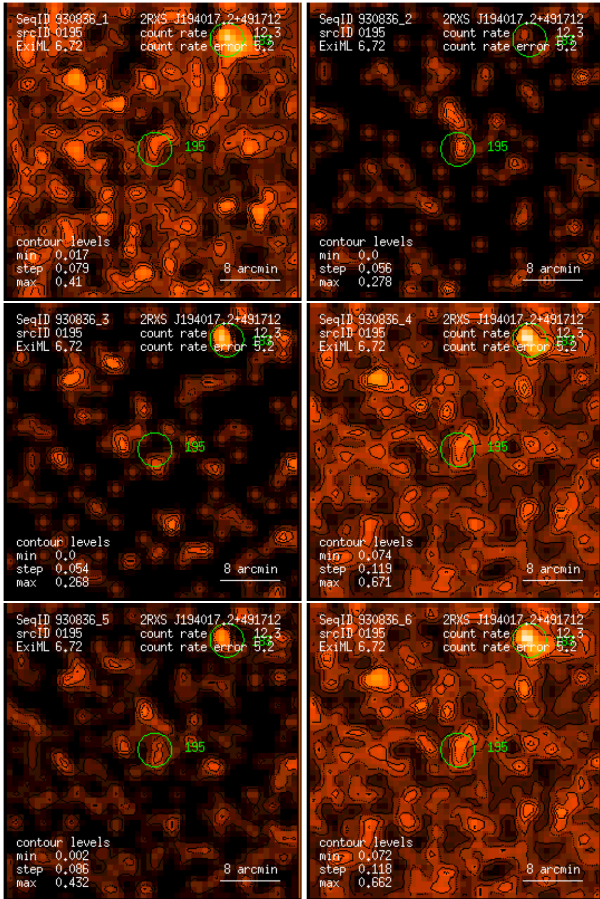
Figure 195: RASS 930836: detection 0195: band rate images, Gaussian filter: (1) PSPC channels 11 – 41, (2) 52 – 90, (3) 91 – 201, (4) 11 – 235, (5) 52 – 201, (6) 11 – 201. Broad band rates in counts/ks. Band rate contour levels in counts/ks/arcmin 2 .
