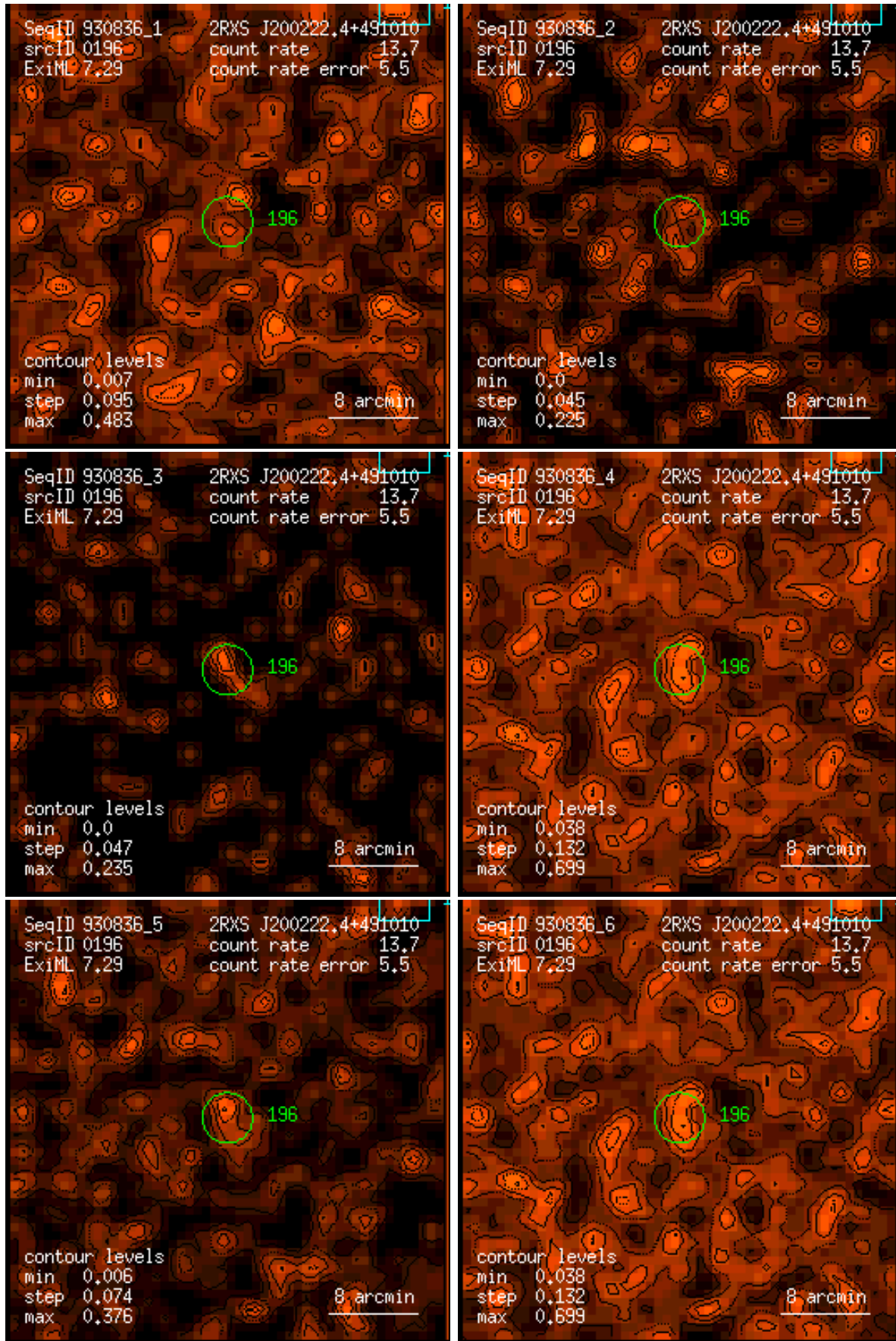
Figure 196: RASS 930836: detection 0196: band rate images, Gaussian filter: (1) PSPC channels 11 – 41, (2) 52 – 90, (3) 91 – 201, (4) 11 – 235, (5) 52 – 201, (6) 11 – 201. Broad band rates in counts/ks. Band rate contour levels in counts/ks/arcmin 2 .
