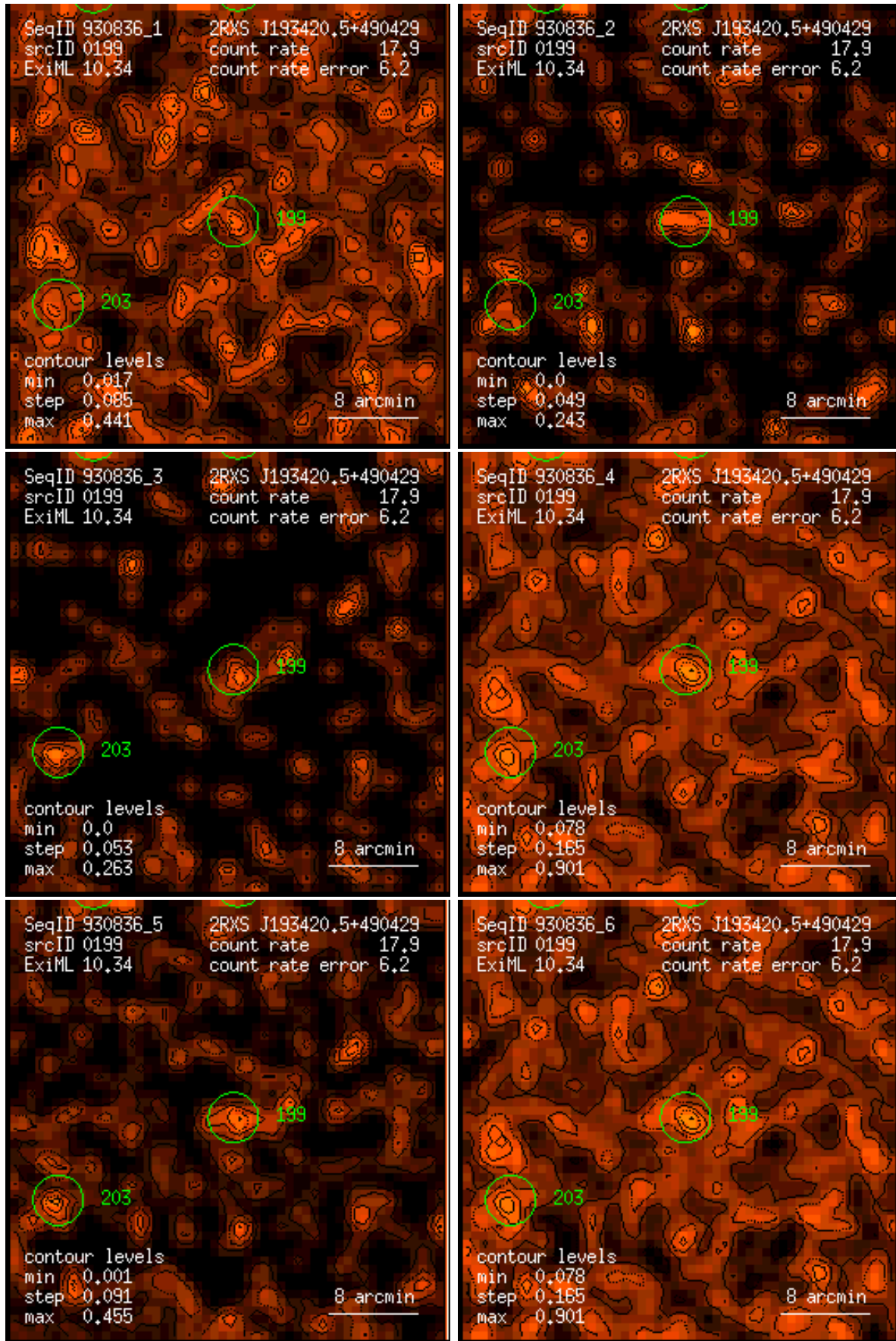
Figure 199: RASS 930836: detection 0199: band rate images, Gaussian filter: (1) PSPC channels 11 – 41, (2) 52 – 90, (3) 91 – 201, (4) 11 – 235, (5) 52 – 201, (6) 11 – 201. Broad band rates in counts/ks. Band rate contour levels in counts/ks/arcmin 2 .
