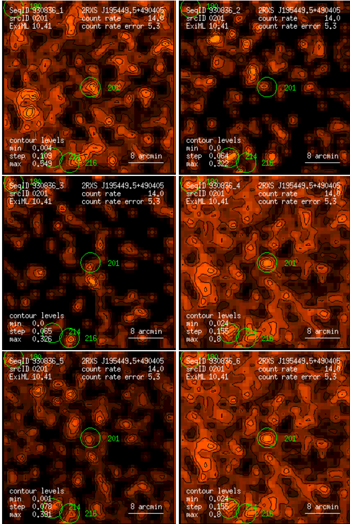
Figure 201: RASS 930836: detection 0201: band rate images, Gaussian filter: (1) PSPC channels 11 – 41, (2) 52 – 90, (3) 91 – 201, (4) 11 – 235, (5) 52 – 201, (6) 11 – 201. Broad band rates in counts/ks. Band rate contour levels in counts/ks/arcmin 2 .
