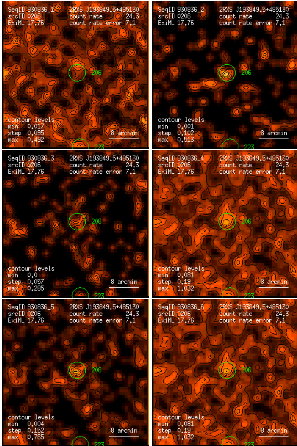
Figure 206: RASS 930836: detection 0206: band rate images, Gaussian filter: (1) PSPC channels 11 – 41, (2) 52 – 90, (3) 91 – 201, (4) 11 – 235, (5) 52 – 201, (6) 11 – 201. Broad band rates in counts/ks. Band rate contour levels in counts/ks/arcmin 2 .
