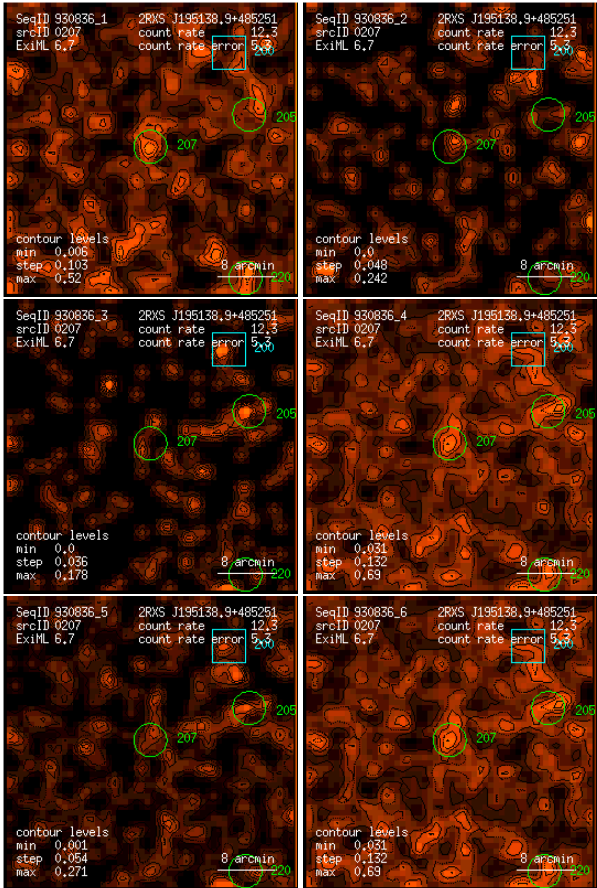
Figure 207: RASS 930836: detection 0207: band rate images, Gaussian filter: (1) PSPC channels 11 – 41, (2) 52 – 90, (3) 91 – 201, (4) 11 – 235, (5) 52 – 201, (6) 11 – 201. Broad band rates in counts/ks. Band rate contour levels in counts/ks/arcmin 2 .
