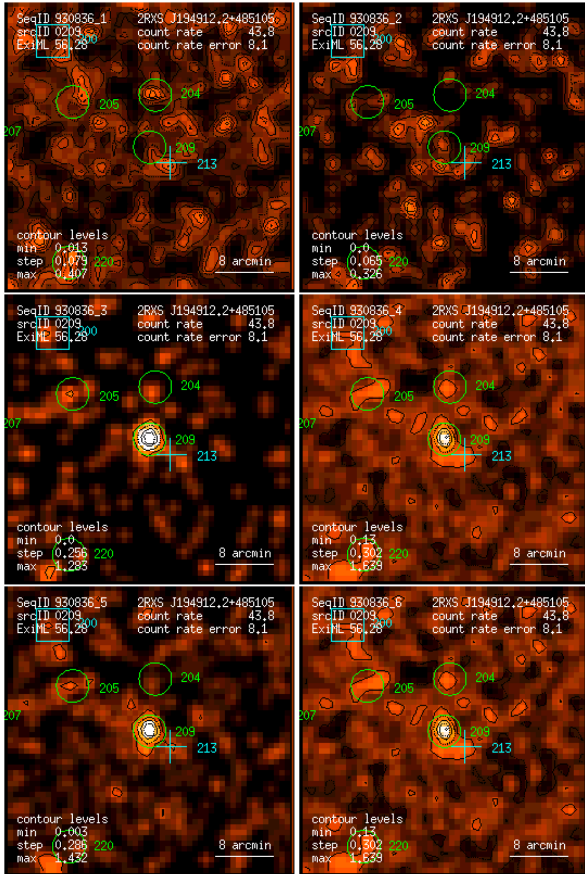
Figure 209: RASS 930836: detection 0209: band rate images, Gaussian filter: (1) PSPC channels 11 – 41, (2) 52 – 90, (3) 91 – 201, (4) 11 – 235, (5) 52 – 201, (6) 11 – 201. Broad band rates in counts/ks. Band rate contour levels in counts/ks/arcmin 2 .
