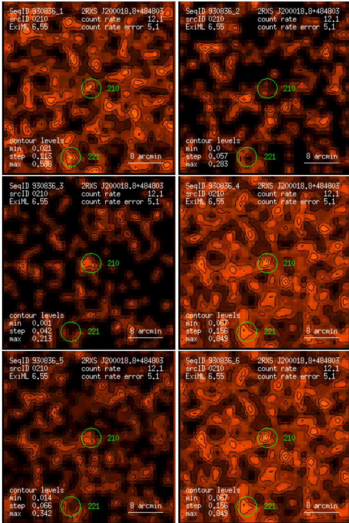
Figure 210: RASS 930836: detection 0210: band rate images, Gaussian filter: (1) PSPC channels 11 – 41, (2) 52 – 90, (3) 91 – 201, (4) 11 – 235, (5) 52 – 201, (6) 11 – 201. Broad band rates in counts/ks. Band rate contour levels in counts/ks/arcmin 2 .
