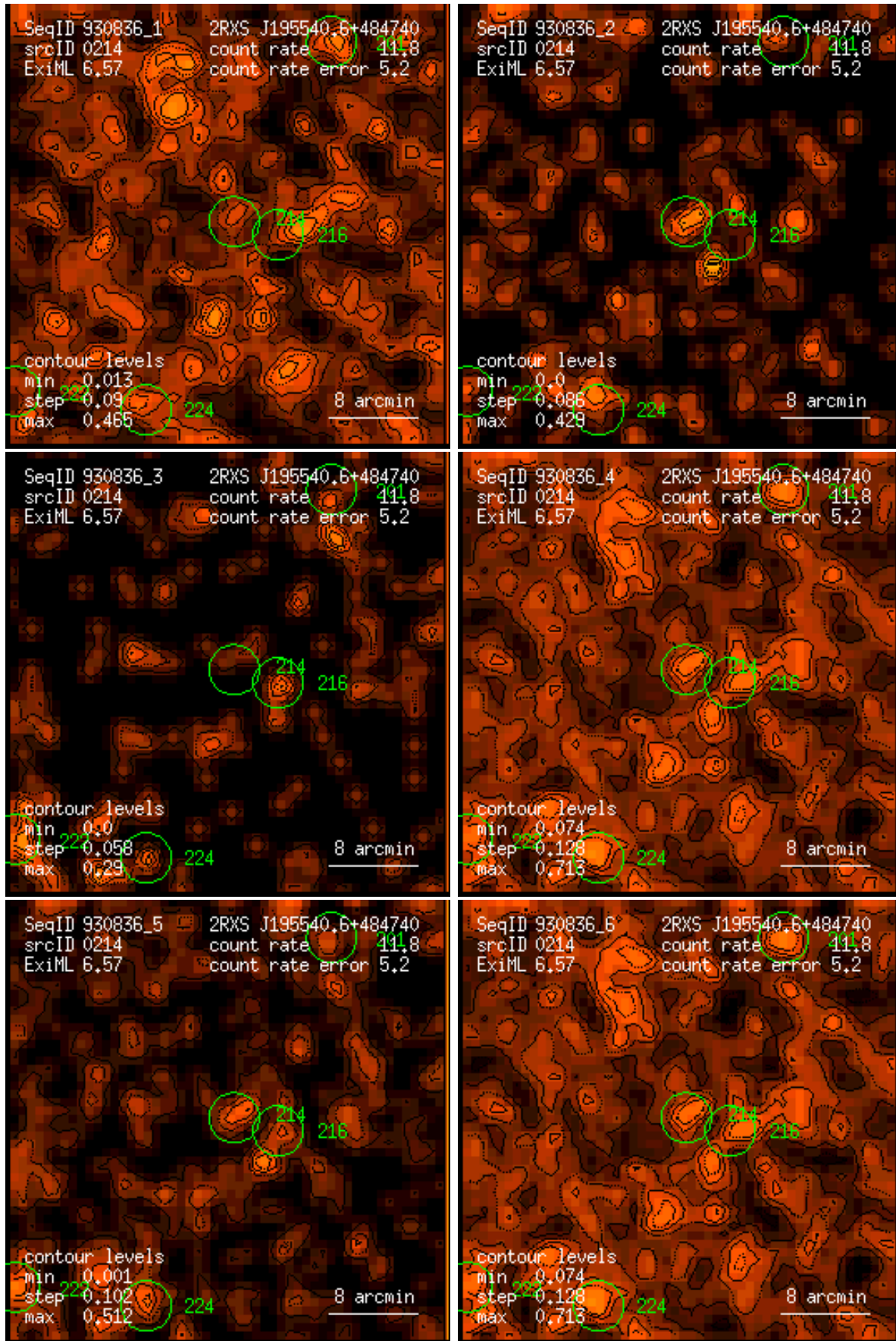
Figure 214: RASS 930836: detection 0214: band rate images, Gaussian filter: (1) PSPC channels 11 – 41, (2) 52 – 90, (3) 91 – 201, (4) 11 – 235, (5) 52 – 201, (6) 11 – 201. Broad band rates in counts/ks. Band rate contour levels in counts/ks/arcmin 2 .
