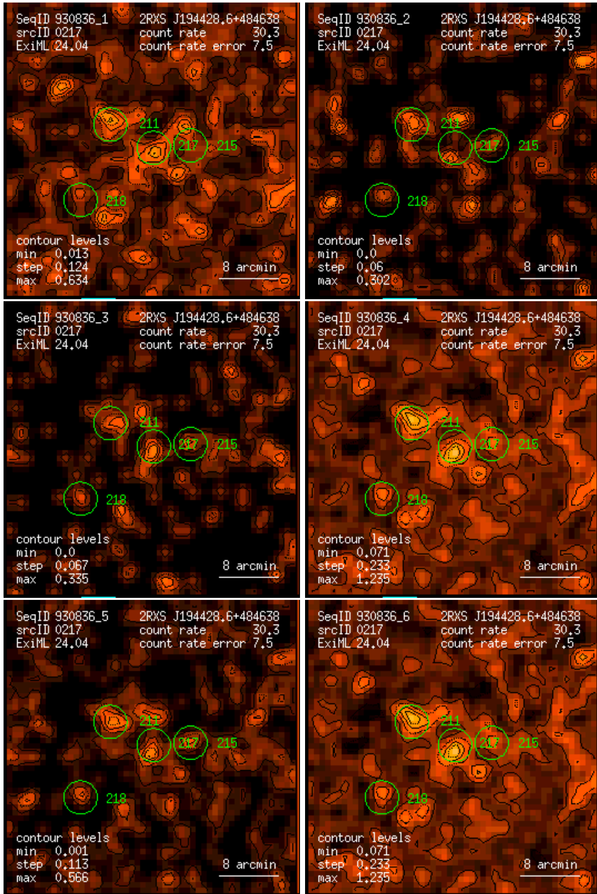
Figure 217: RASS 930836: detection 0217: band rate images, Gaussian filter: (1) PSPC channels 11 – 41, (2) 52 – 90, (3) 91 – 201, (4) 11 – 235, (5) 52 – 201, (6) 11 – 201. Broad band rates in counts/ks. Band rate contour levels in counts/ks/arcmin 2 .
