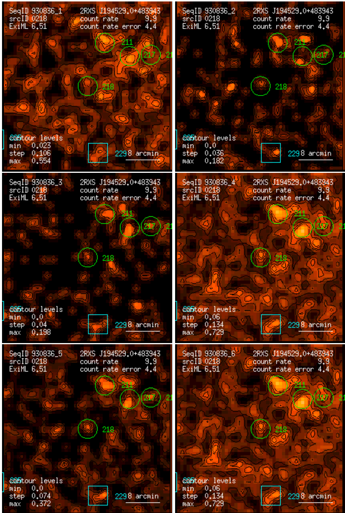
Figure 218: RASS 930836: detection 0218: band rate images, Gaussian filter: (1) PSPC channels 11 – 41, (2) 52 – 90, (3) 91 – 201, (4) 11 – 235, (5) 52 – 201, (6) 11 – 201. Broad band rates in counts/ks. Band rate contour levels in counts/ks/arcmin 2 .
