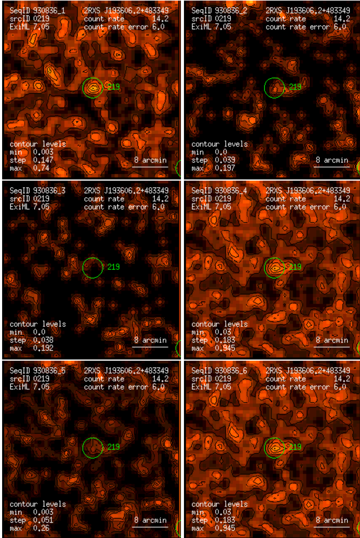
Figure 219: RASS 930836: detection 0219: band rate images, Gaussian filter: (1) PSPC channels 11 – 41, (2) 52 – 90, (3) 91 – 201, (4) 11 – 235, (5) 52 – 201, (6) 11 – 201. Broad band rates in counts/ks. Band rate contour levels in counts/ks/arcmin 2 .
