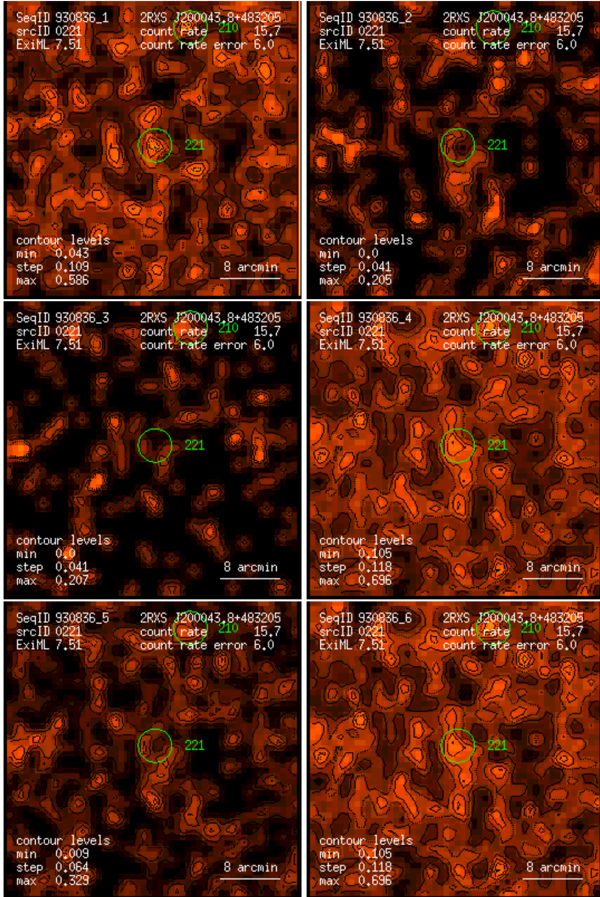
Figure 221: RASS 930836: detection 0221: band rate images, Gaussian filter: (1) PSPC channels 11 – 41, (2) 52 – 90, (3) 91 – 201, (4) 11 – 235, (5) 52 – 201, (6) 11 – 201. Broad band rates in counts/ks. Band rate contour levels in counts/ks/arcmin 2 .
