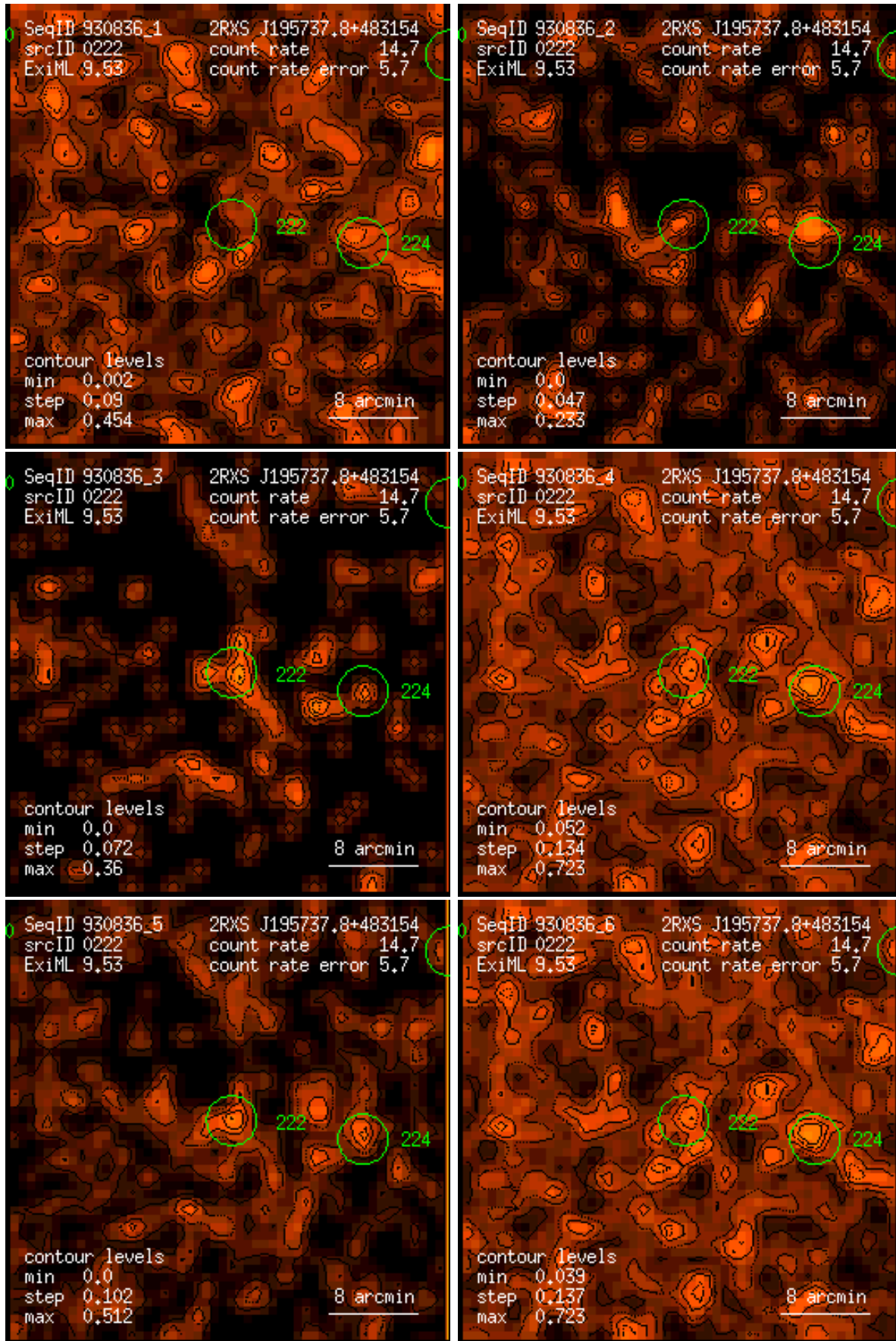
Figure 222: RASS 930836: detection 0222: band rate images, Gaussian filter: (1) PSPC channels 11 – 41, (2) 52 – 90, (3) 91 – 201, (4) 11 – 235, (5) 52 – 201, (6) 11 – 201. Broad band rates in counts/ks. Band rate contour levels in counts/ks/arcmin 2 .
