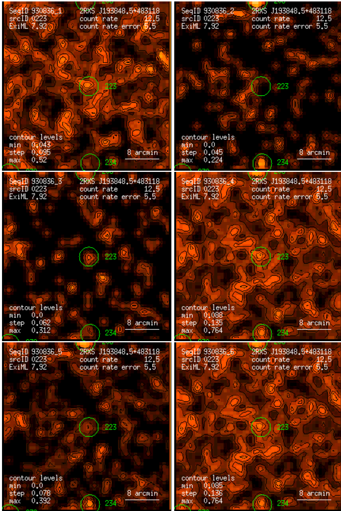
Figure 223: RASS 930836: detection 0223: band rate images, Gaussian filter: (1) PSPC channels 11 – 41, (2) 52 – 90, (3) 91 – 201, (4) 11 – 235, (5) 52 – 201, (6) 11 – 201. Broad band rates in counts/ks. Band rate contour levels in counts/ks/arcmin 2 .
